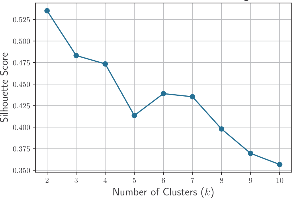
Euclidean distance with variance weights
