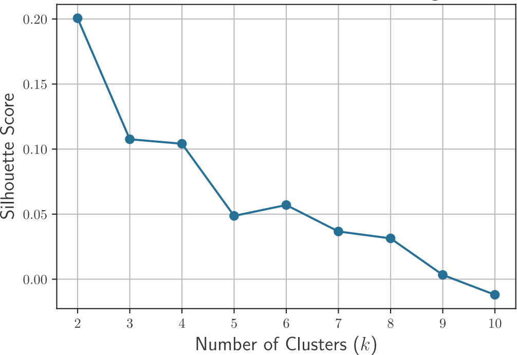
Euclidean distance with variance weights
