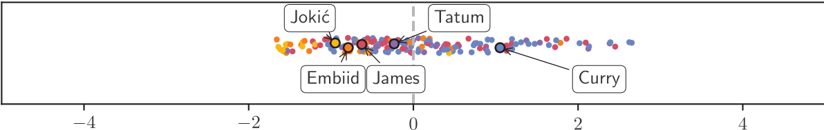
Scores c_1
