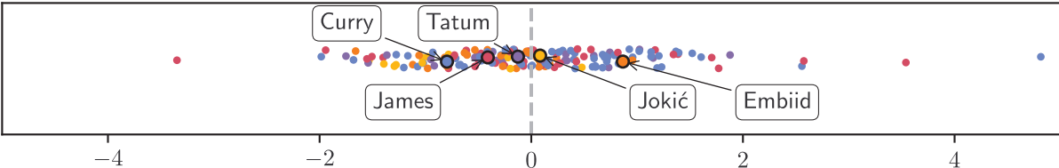
Scores c_2
