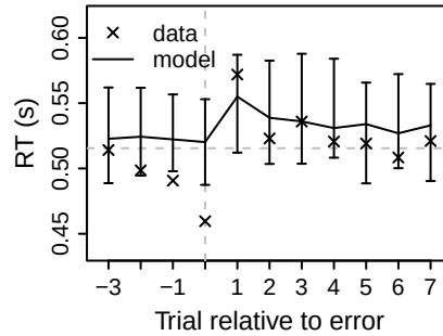
Figure 29: Quality of fit of error-related effects by a WDM that allows thresholds to vary with accuracy memory. x-axes depict trial number relative to the error (trial 0); crosses are (group-averaged) mean RTs, error bars are 95% credible intervals of the models. Horizontal dashed lines indicate the mean RT.
