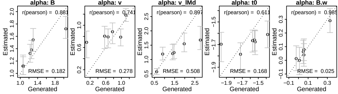
Figure 14: Parameter recovery results for the subject-level parameters. Estimated parameters (y-axis) are plotted against data-generating (x-axis). Error bars indicate 95% credible intervals, circles are on the median posterior, and diagonal lines is the identity. Pearson correlation between data-generating and posterior median. RMSE = root mean squared error.
