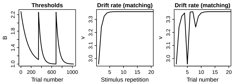
Figure 18: Effect of specifying multiple trends with parameters that vary between blocks (left) or conditions (middle, right).
