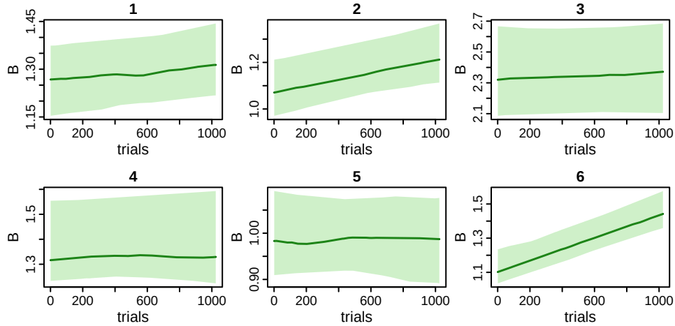
Figure 13: Estimated thresholds (B) as a function of trial number. Each panel corresponds to one participant (titles). Green shaded areas correspond to the 95% credible interval, the dark green line corresponds to the mean across posterior predictive datasets.
