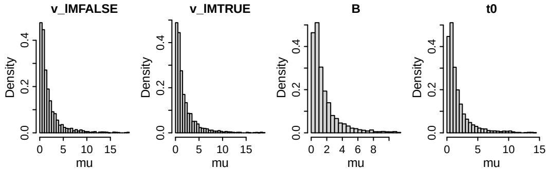
Figure 2: Implied default priors for the group-level mean parameters of the baseline RDM. v_{1MTRUE} and v_{1MFALSE} refer to the drift rate of the accumulators matching ('correct') and mismatching ('error') the stimulus, respectively; B to the threshold, and t_0 to the non-decision time.
