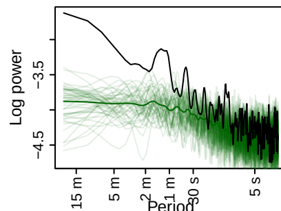
Figure 30: Group-averaged power spectrum of the RT data (black line) and model posterior predictives (green). Each individual green line is one posterior predictives’ (group-averaged) power spectrum; the dark green line averages across posterior predictives.
