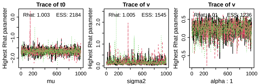
Figure 3: Trace plots of the sampled parameters with highest Rhat values (i.e., worst convergence) at the group-level mean (left, \mu ), the group-level variance (middle, \sigma^2 ), and the subject-level ( \alpha ; in this case, subject number 1). ESS = effective sample size.
