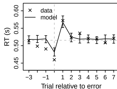
Figure 28: Quality of fit of error-related effects by an RDM that allows urgency to vary with accuracy memory. x-axes depict trial number relative to the error (trial 0); crosses are (group-averaged) mean RTs, error bars are 95% credible intervals of the models. Horizontal dashed lines indicate the mean RT.
