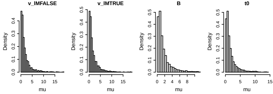
Figure 1: Implied default priors for the group-level mean parameters of the baseline RDM model. v_1MTRUE and v_1MFALSE refer to the drift rate of the accumulators matching ('correct') and mismatching ('error') the stimulus, respectively; B to the threshold, and t0 to the non-decision time.
