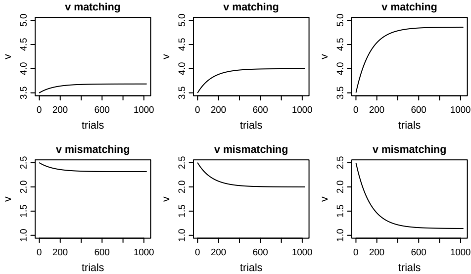
Figure 13: Demonstration of enforcing a direction of an effect. Irrespective of the sign of v\_lMd.w (-1 for column 1, 0 for column 2, and 1 for column 3), the difference between the matching and mismatching accumulator's drift rate increases over trials when v\_lMd.w is estimated on the log scale and the increasing exponential kernel is used.
