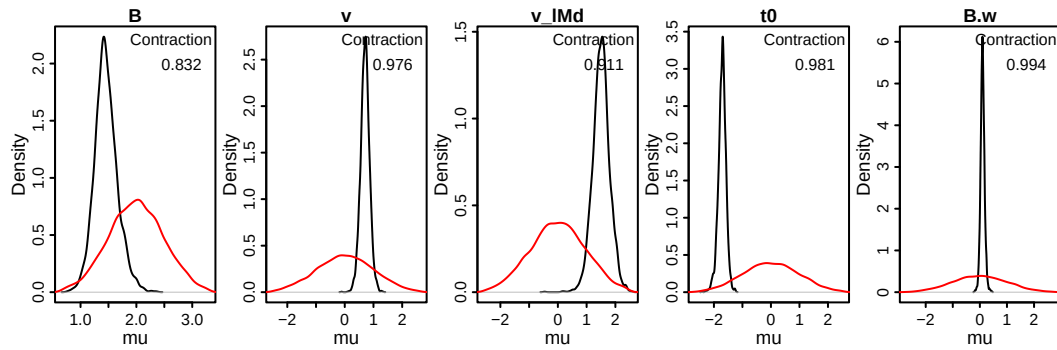
Figure 8: Posterior density (black) and prior density (red) of sampled group-level mean parameters of the RDM with a linear trend. Contraction indicates the reduction of uncertainty in the posterior versus the prior (1 minus the ratio of the posterior to prior variance).
