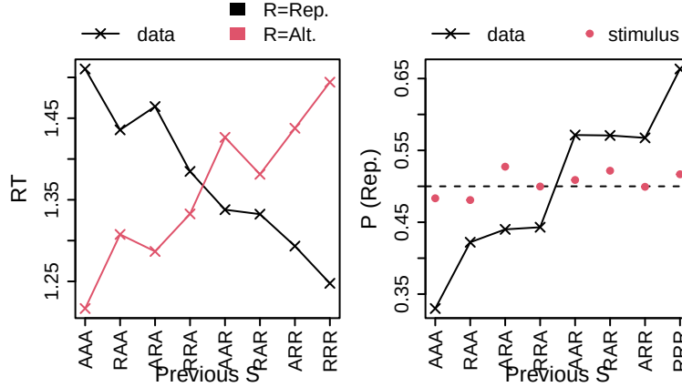
Figure 19: Effects of local stimulus (S) repetition history on response times (left) and response (R) probability (right). X-axis labels indicate the three most recent trials’ stimuli, coded as whether they repeated (R) or alternated (A) the preceding trial (e.g., AAA = alternate, alternate, alternate, AAR = alternate, alternate, repeat; the right-most letter in the string indicates the most recent trial). Crosses indicate data. Red circles in the right plot indicate the probability of the stimulus repeating the previous stimulus, which is an important quality check.
