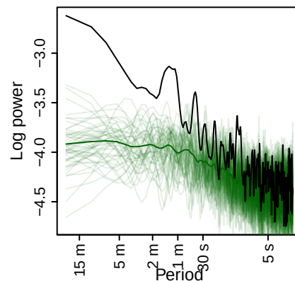
Figure 24: Group-averaged power spectrum of the RT data (black line) and model posterior predictives (green). Each individual green line is one posterior predictives’ (group-averaged) power spectrum; the dark green line averages across posterior predictives.
