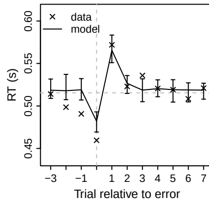
Figure 22: Quality of fit of error-related effects by an RDM that allows urgency to vary with accuracy memory. x-axes depict trial number relative to the error (trial 0); crosses are (group-averaged) mean RTs, error bars are 95% credible intervals of the models. Horizontal dashed lines indicate the mean RT.
