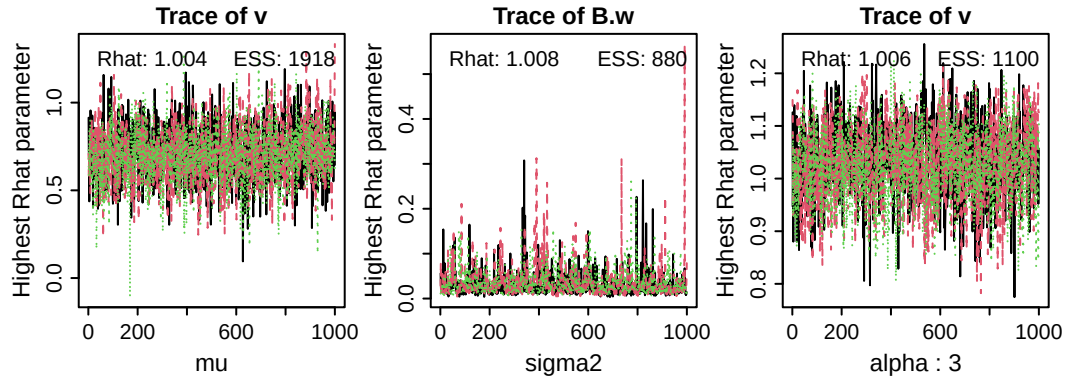
Figure 7: Trace plots of the sampled parameters with highest Rhat values (i.e., worst convergence) at the group-level mean (left, \mu ), the group-level variance (middle, \sigma^2 ), and the subject-level ( \alpha ; in this case, subject number 3). ESS = effective sample size.
