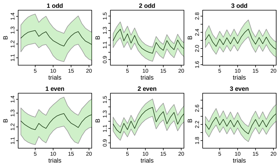
Figure 17: Estimated trialwise thresholds of the accumulator corresponding to responding odd (top) and even (bottom) for the first three participants (columns). Green shaded areas indicate the 95% credible interval.
