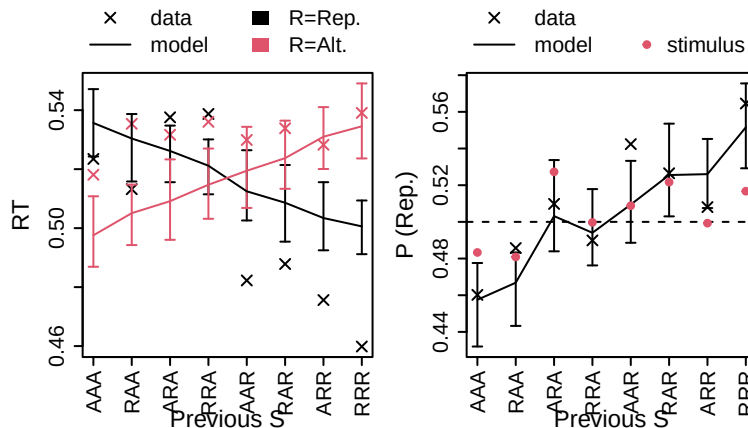
Figure 20: Effects of local stimulus (S) repetition history on response times (left) and response (R) probability (right). X-axis labels indicate the three most recent trials’ stimuli, coded as whether they repeated (R) or alternated (A) the preceding trial (e.g., AAA = alternate, alternate, alternate, AAR = alternate, alternate, repeat; the right-most letter in the string indicates the most recent trial). Crosses indicate data, model predictions are indicated by error bars (95% credible intervals), and lines connect medians. Red circles in the right plot indicate the probability of the stimulus repeating the previous stimulus, which is an important quality check.
