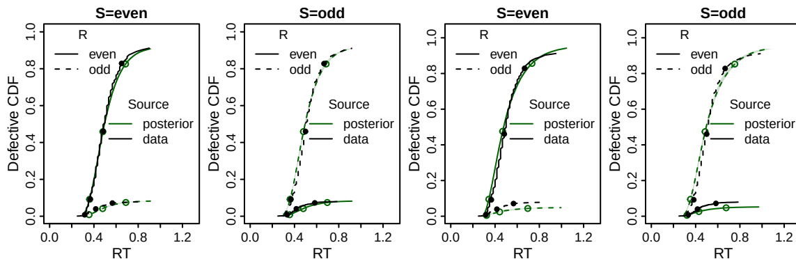
Figure 4: Defective cumulative density plots of the baseline RDM (left two columns) and WDM (right two columns). Circles indicate the 10th, 50th, and 90ths quantiles of the response time distributions for each response type R (solid = 'even', dotted = 'odd') in both conditions of the stimulus S (panels) for the data (black) and posterior predictives (green). The cumulative density functions are made defective as they sum to the proportion of each choice (rather than 1).
