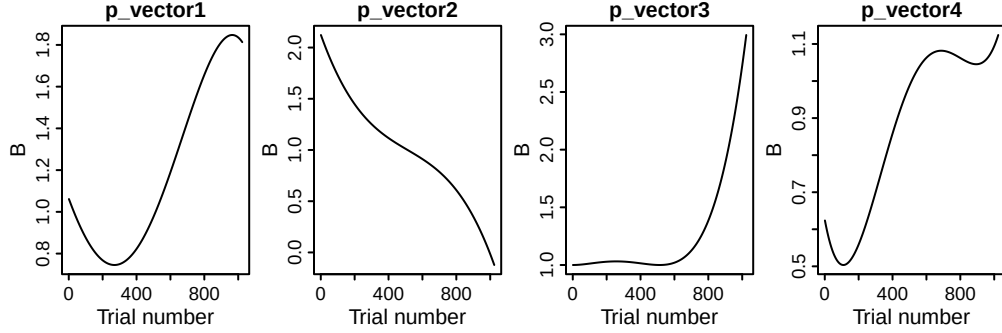
Figure 13: Illustration of the flexibility of the polynomial kernel: With four different (arbitrarily chosen) parameter sets, widely different shapes of trends can be obtained. Here, they are visualised as trends on thresholds B , but they can be on any parameter.
