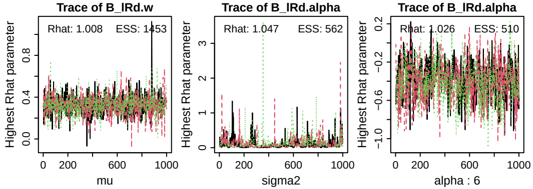
Figure 14: Trace plots of the sampled parameters with highest Rhat values (i.e., worst convergence) at the group-level mean (left, \mu ), the group-level variance (middle, \sigma^2 ), and the subject-level ( \alpha ; in this case, subject number 6). ESS = effective sample size.
