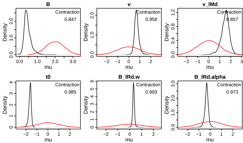
Figure 15: Posterior density (black) and prior density (red) of sampled group-level mean parameters of the RDM with an SM mechanism. Contraction indicates the reduction of uncertainty in the posterior versus the prior (1 minus the ratio of the posterior to prior variance).
