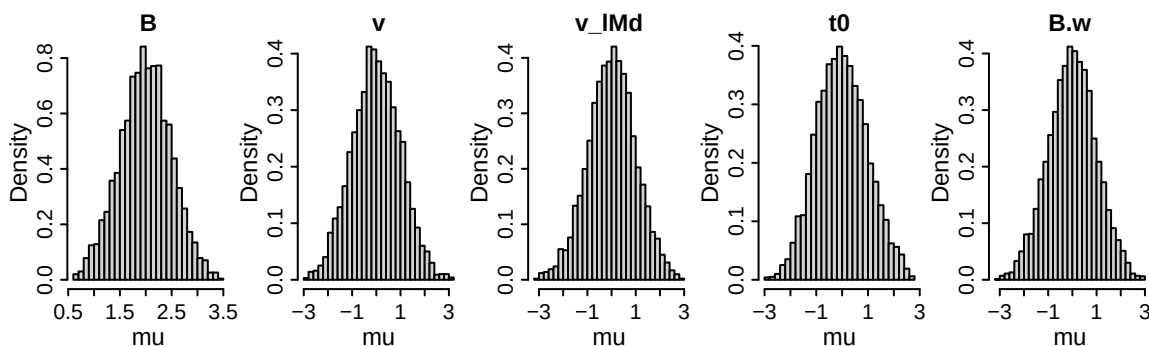
Figure 6: Prior distributions for the group-level mean parameters of the RDM with a linear trend, with the threshold B sampled in the natural scale.
