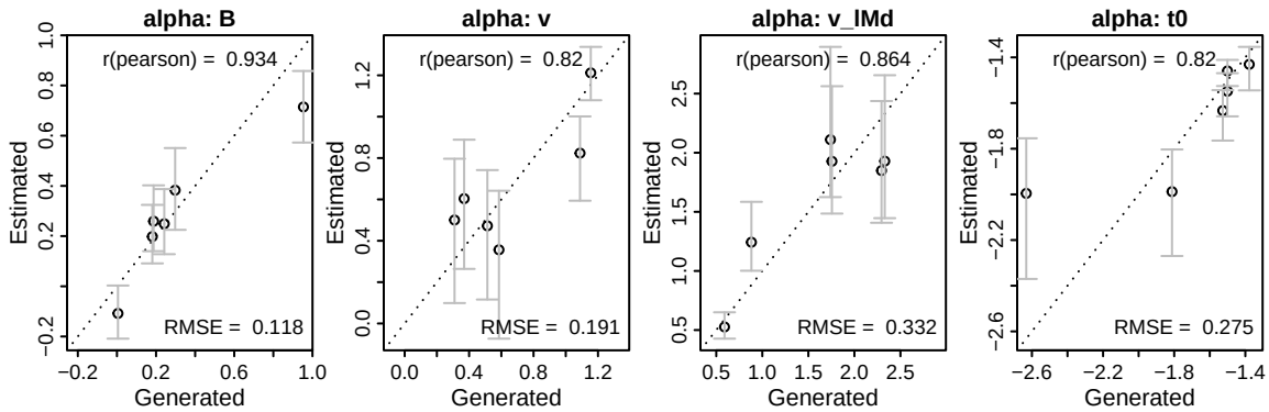
Figure 5: Parameter recovery results for the subject-level parameters. Estimated parameters (y-axis) are plotted against data-generating (x-axis). Error bars indicate 95% credible intervals, circles are on the median posterior, and diagonal lines is the identity. Pearson correlation between data-generating and posterior median. RMSE = root mean squared error.
