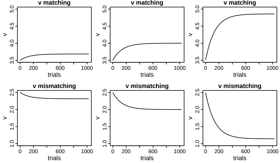
Figure 11: Demonstration of enforcing a direction of an effect. Irrespective of the sign of v\_lmd.w (-1 for column 1, 0 for column 2, and 1 for column 3), the difference between the matching and mismatching accumulator’s drift rate increases over trials when v\_lmd.w is estimated on the log scale and the increasing exponential kernel is used.
