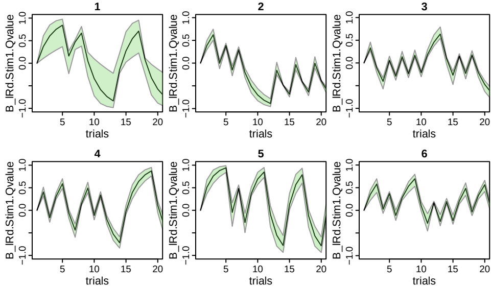
Figure 18: Estimated Q-values corresponding to the SM mechanism for all six participants (panels). Green shaded areas indicate the 95% credible interval.
