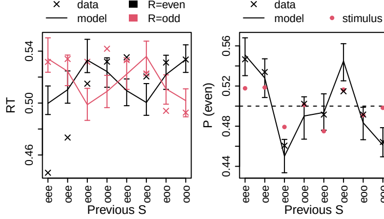
Figure 21: Effects of local stimulus (S) history on response times (left) and response (R) probability (right). X-axis labels indicate the three most recent trials' stimuli (e.g., eee = even, even even, eeo = even, even, odd; the right-most letter in the string indicates the most recent trial). Crosses indicate data, model predictions (in this case, the DDM with a drift rate effect of stimulus memory) are indicated by error bars (95% credible intervals), and lines connect medians. Red circles in the right plot indicate the probability of the stimulus, which is an important quality check.
