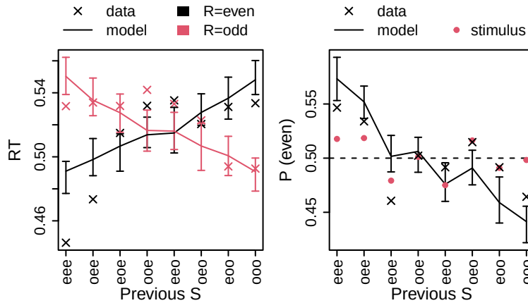
Figure 16: Effects of local stimulus (S) history on response times (left) and response (R) probability (right). X-axis labels indicate the three most recent trials' stimuli (e.g., eee = even, even even, eeo = even, even, odd; the right-most letter in the string indicates the most recent trial). Crosses indicate data, model predictions are indicated by error bars (95% credible intervals), and lines connect medians. Red circles in the right plot indicate the probability of the stimulus, which is an important quality check.
