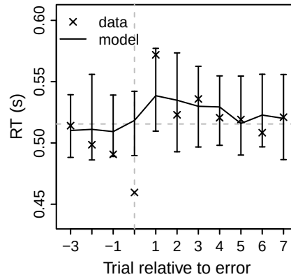
Figure 23: Quality of fit of error-related effects by a WDM that allows thresholds to vary with accuracy memory. x-axes depict trial number relative to the error (trial 0); crosses are (group-averaged) mean RTs, error bars are 95% credible intervals of the models. Horizontal dashed lines indicate the mean RT.
