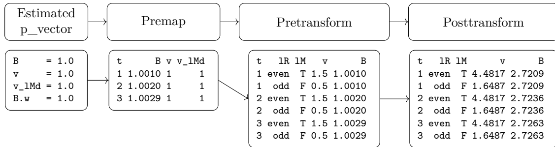
Figure 7: Illustration of parameter mapping and transformation in EMC2 . The estimated parameter vector is first mapped, then transformed. In the illustration, only drift rates v and thresholds B are shown. In this example, the trend is applied premap , which leads the threshold to increase with trials ( t ). After mapping, the parameters are expanded to each design cell, with in this example two accumulators per trial (one for each latent response lR , and one matches the stimulus lM=T ). Finally, the parameters are transformed to the natural scale. Since in this example, a linear trend is applied premap , this leads to an exponentially increasing trend posttransform .
