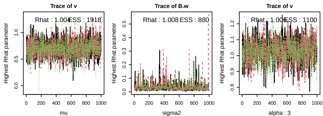
Figure 9: Trace plots of the sampled parameters with highest Rhat values (i.e., worst convergence) at the group-level mean (left, \mu ), the group-level variance (middle, \sigma^2 ), and the subject-level ( \alpha ; in this case, subject number 3). ESS = effective sample size.
