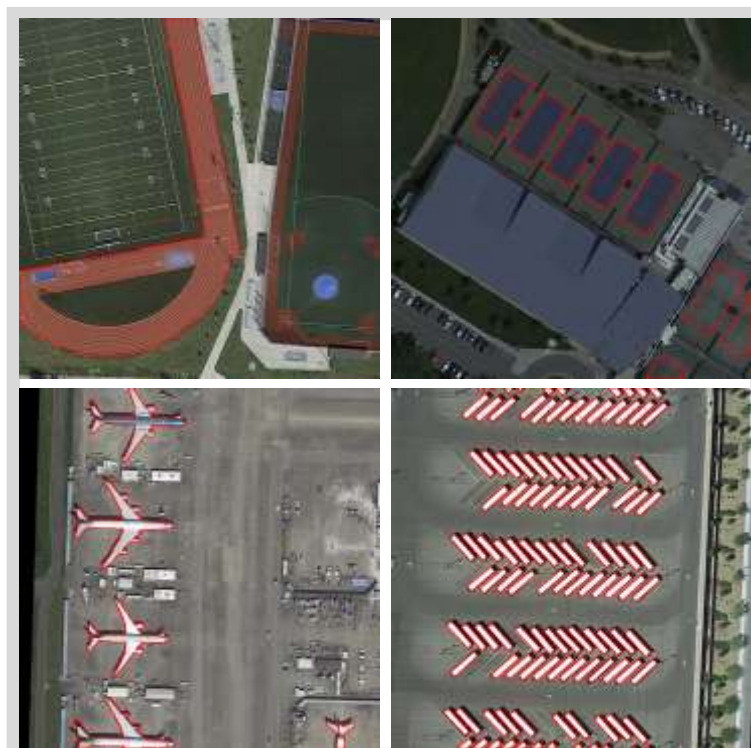
iSAID
