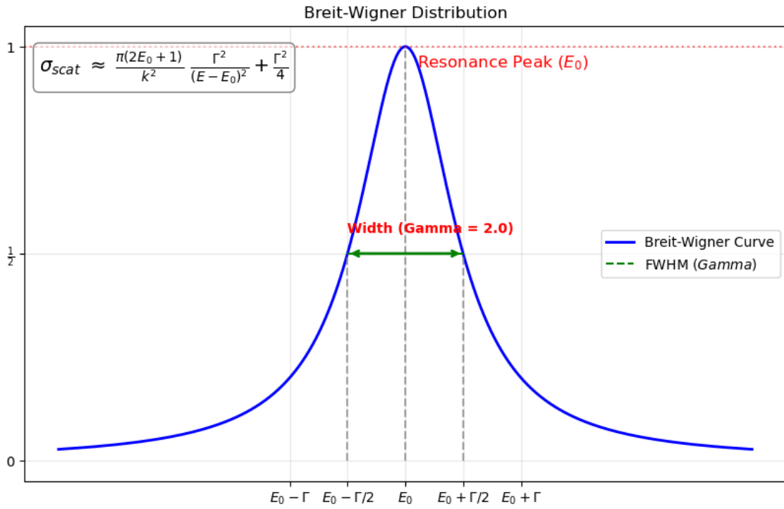
Figure A.3: Breit-Wigner distribution
