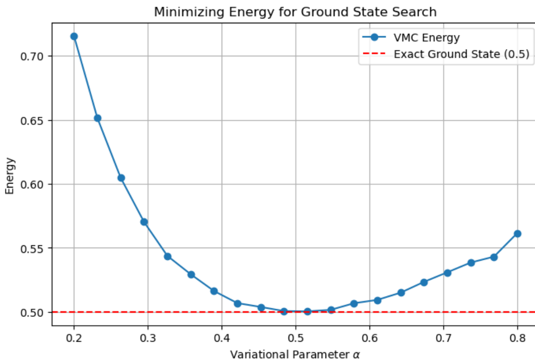
Figure A.1: Minimizing energy for a ground-state
