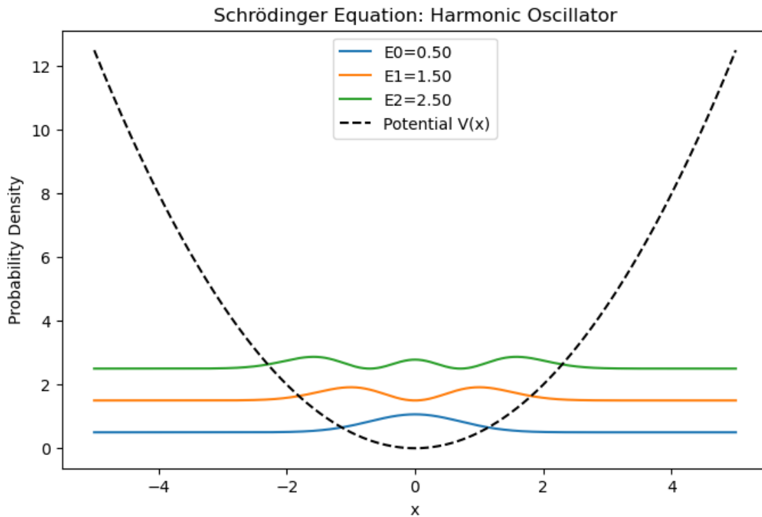
Figure 3.3: This is a figure of the Quantum Harmonic Oscillator. It is defined by E_n = (n + \frac{1}{2})\hbar\omega
