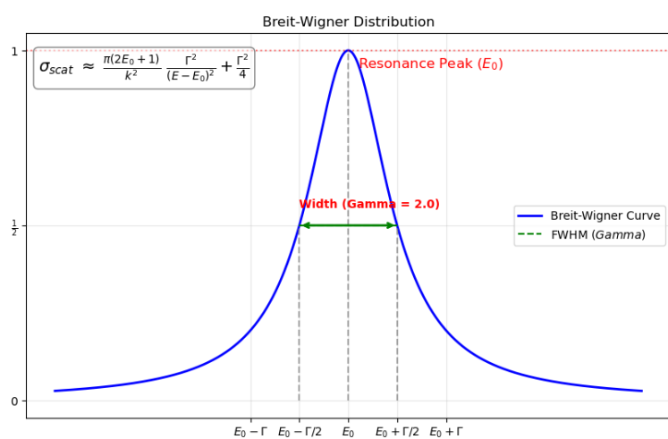
Figure 7.3: Breit-Wigner distribution
