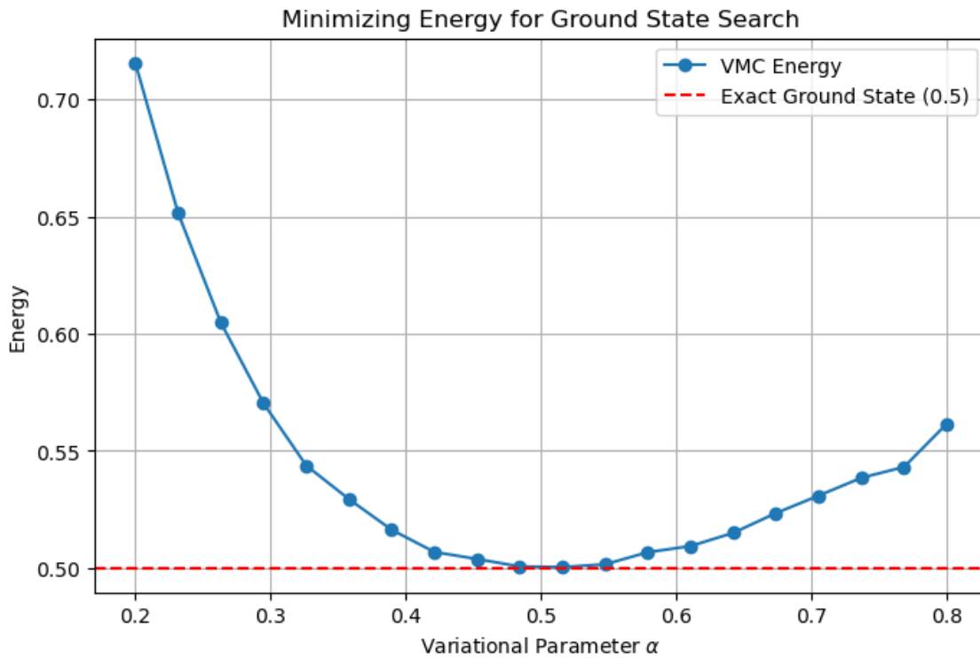
Figure B.1: Minimizing energy for a ground-state
