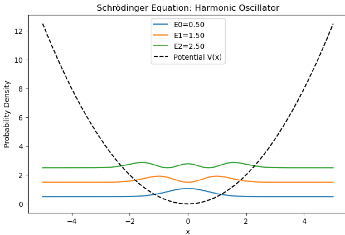
Figure 1.3: This is a figure of the Quantum Harmonic Oscillator. It is defined by E_n = (n + \frac{1}{2})\hbar\omega
