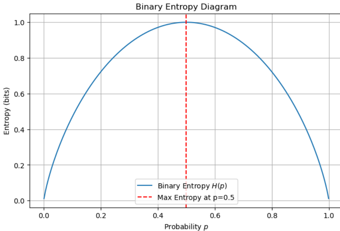
Figure 1.1: Binary Entropy
