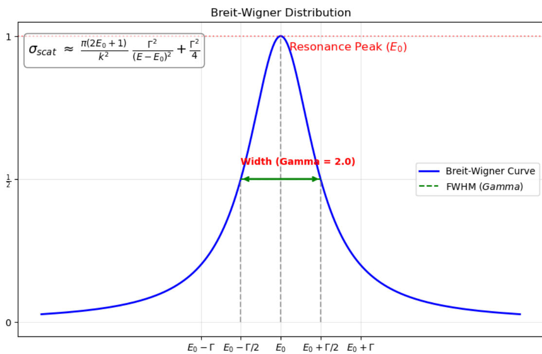
Figure B.3: Breit-Wigner distribution
