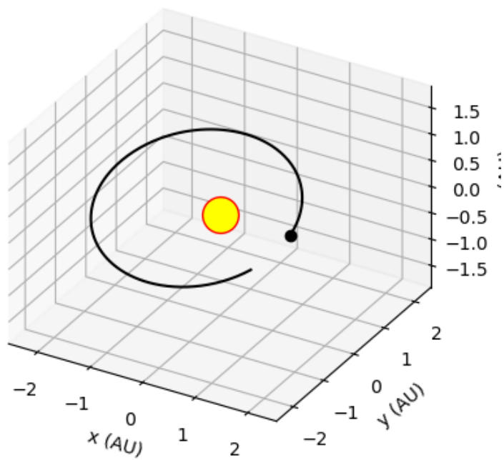
Figure 3.2: vector pointing towards the Sun
