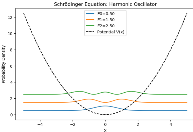
Figure 4.1: This is a figure of the Quantum Harmonic Oscillator. It is defined by E_n = (n + \frac{1}{2})\hbar\omega
