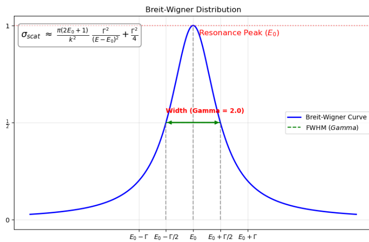
Figure 8.3: Breit-Wigner distribution
