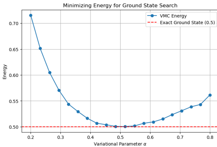
Figure 8.1: Minimizing energy for a ground-state
