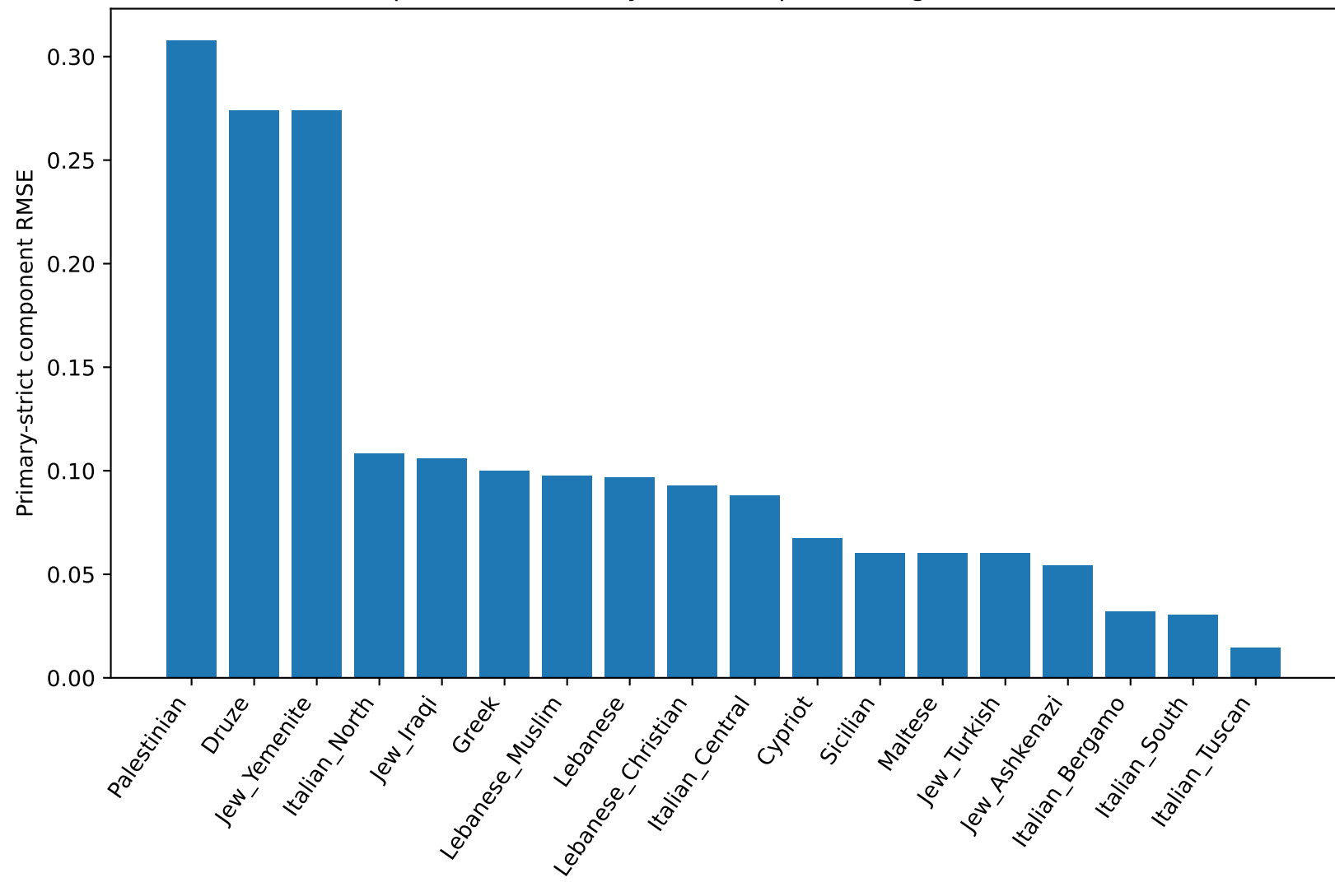
Population sensitivity after component alignment, K=5
