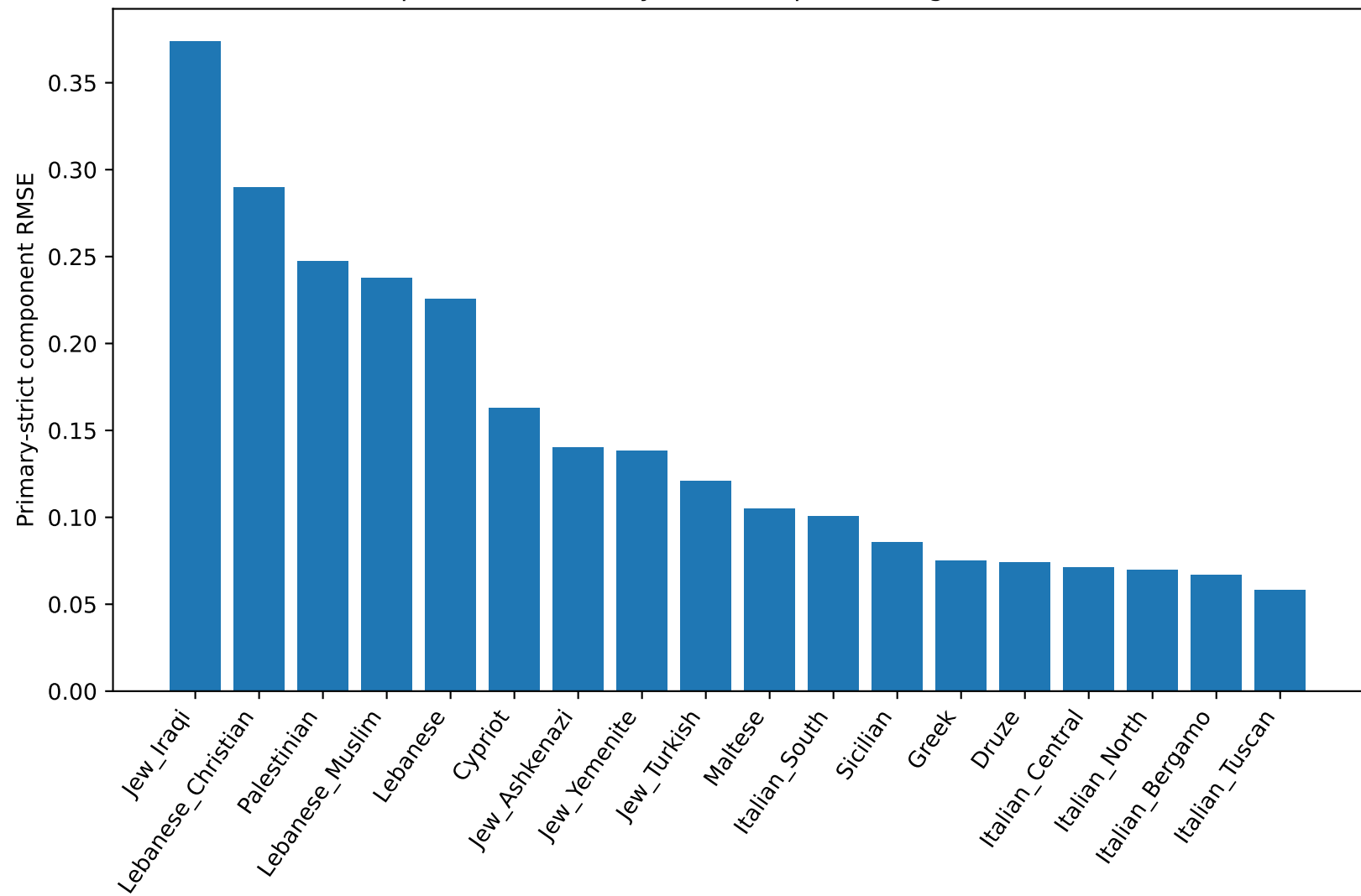
Population sensitivity after component alignment, K=8
