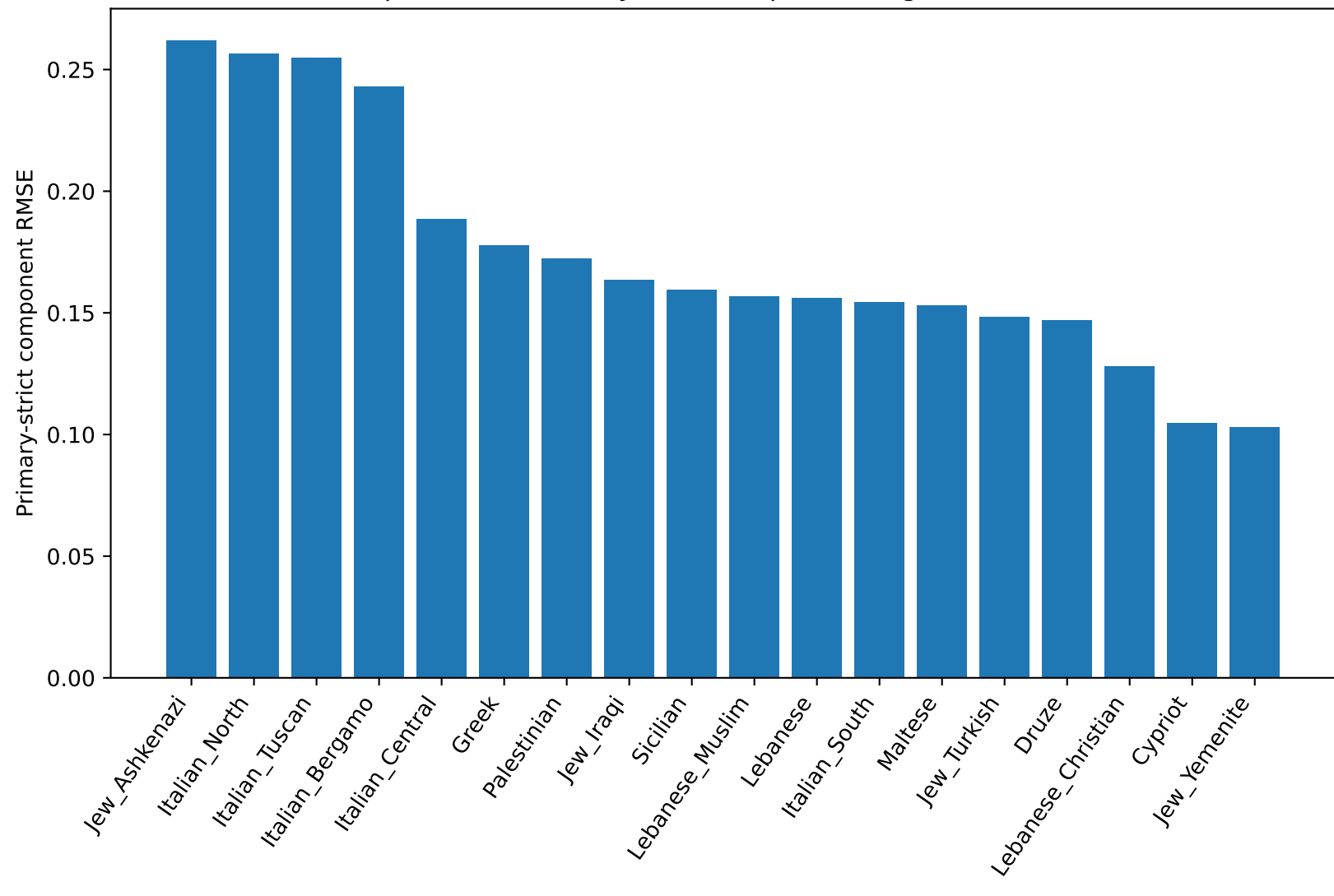
Population sensitivity after component alignment, K=11
