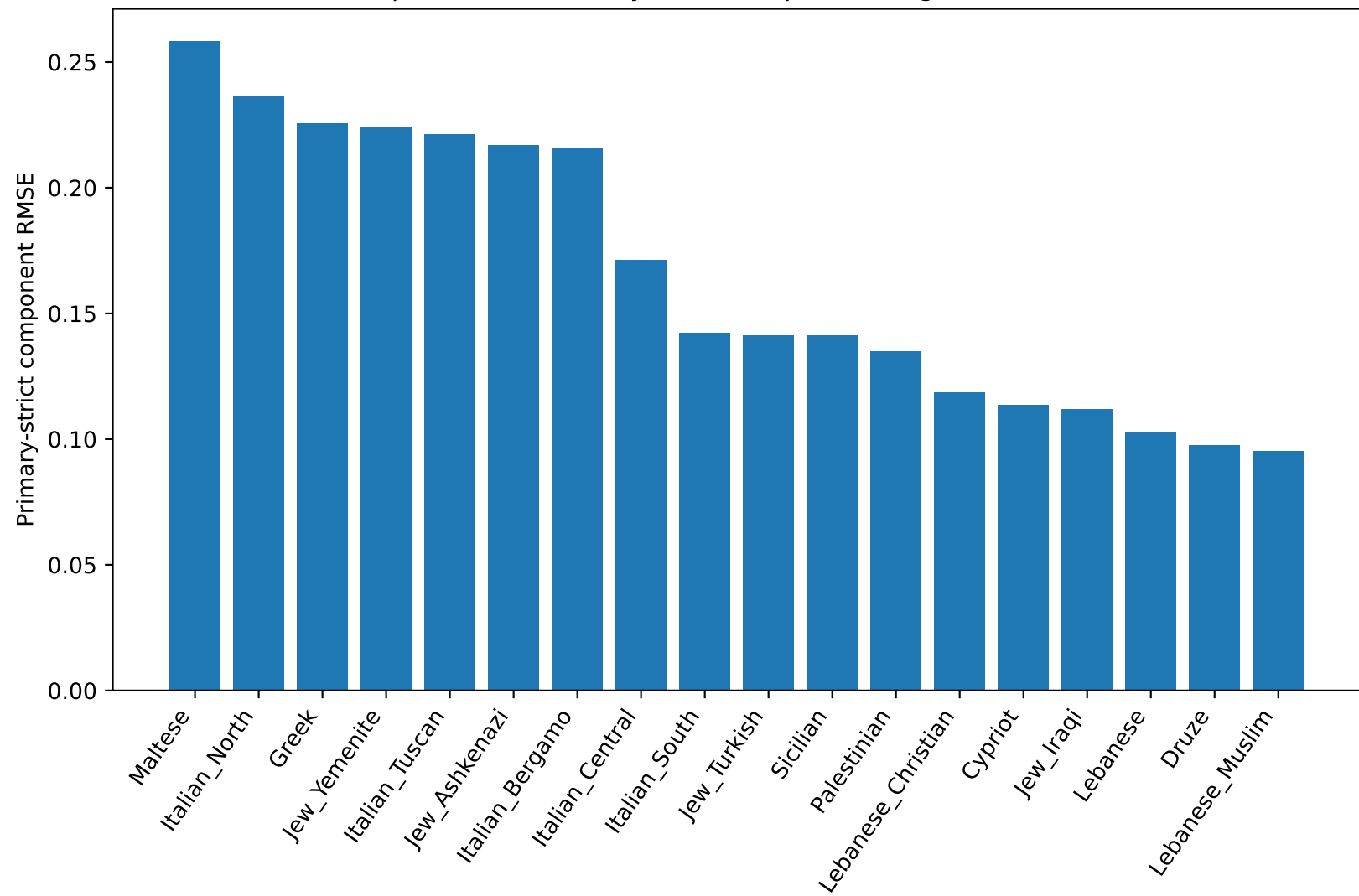
Population sensitivity after component alignment, K=12
