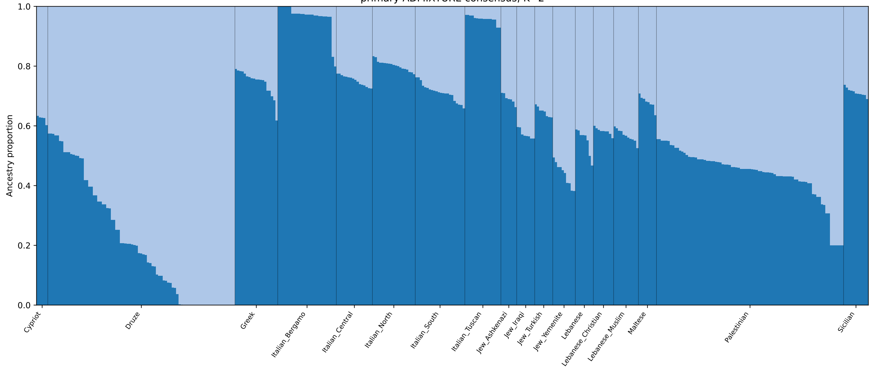
primary ADMIXTURE consensus, K=2
