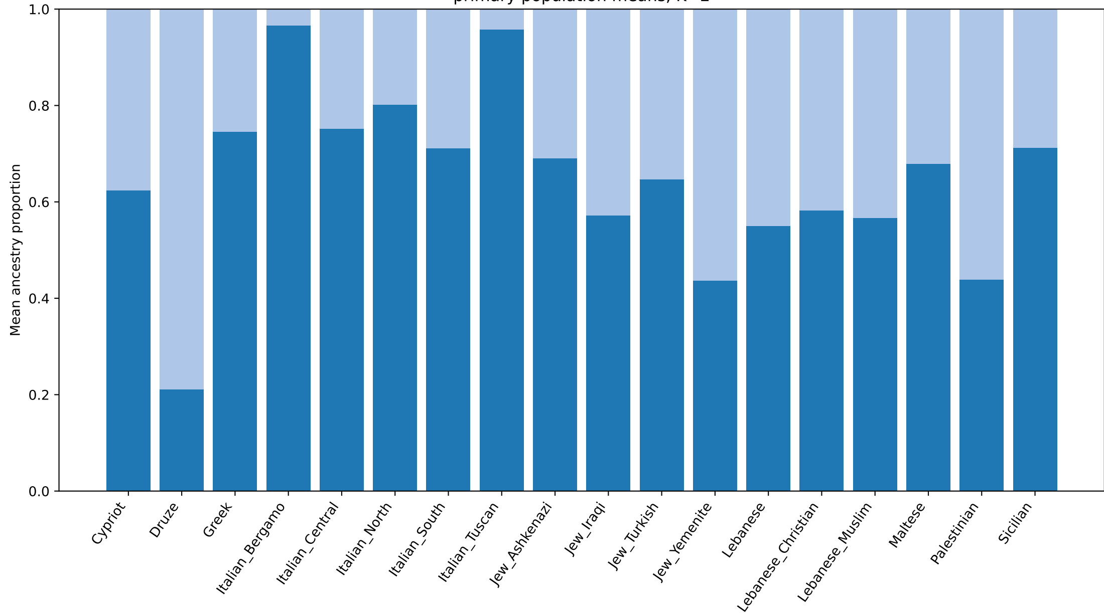
primary population means, K=2
