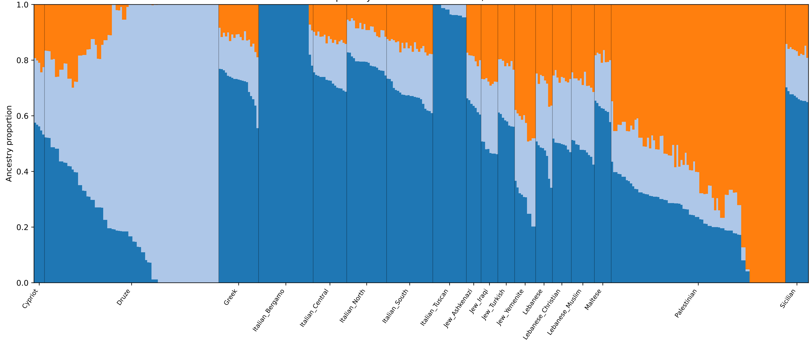
primary ADMIXTURE consensus, K=3
