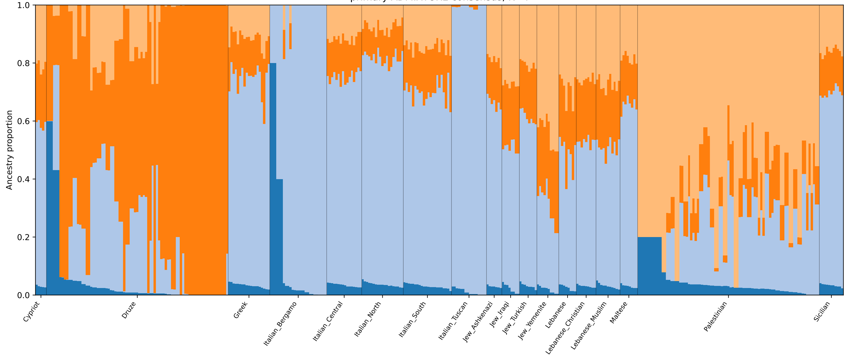
primary ADMIXTURE consensus, K=4
