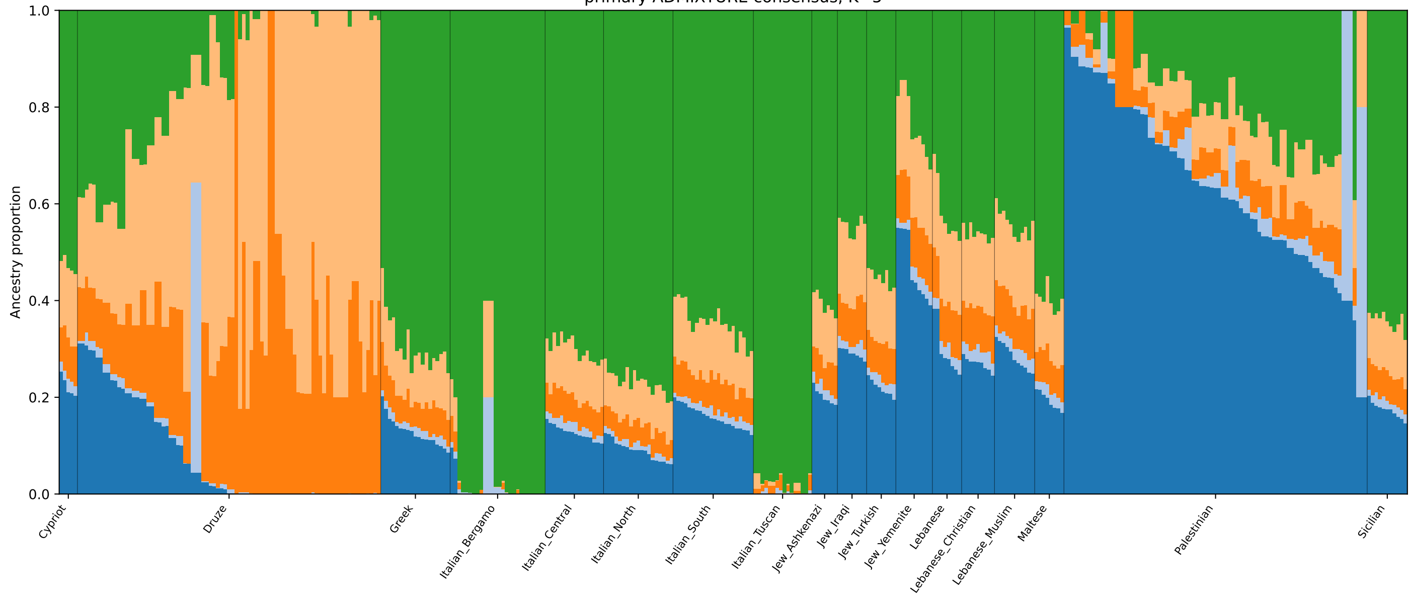
primary ADMIXTURE consensus, K=5
