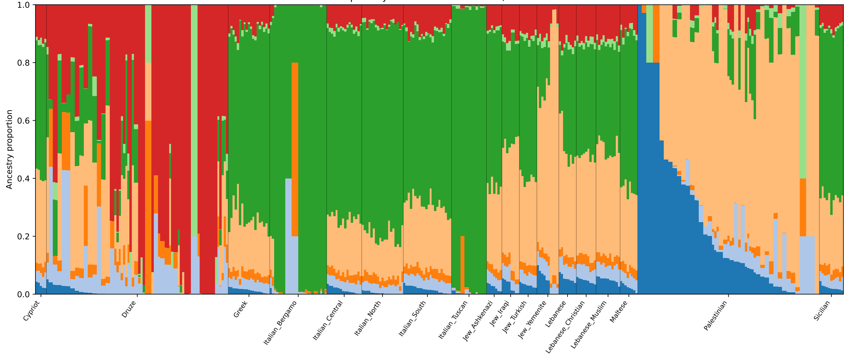
primary ADMIXTURE consensus, K=7
