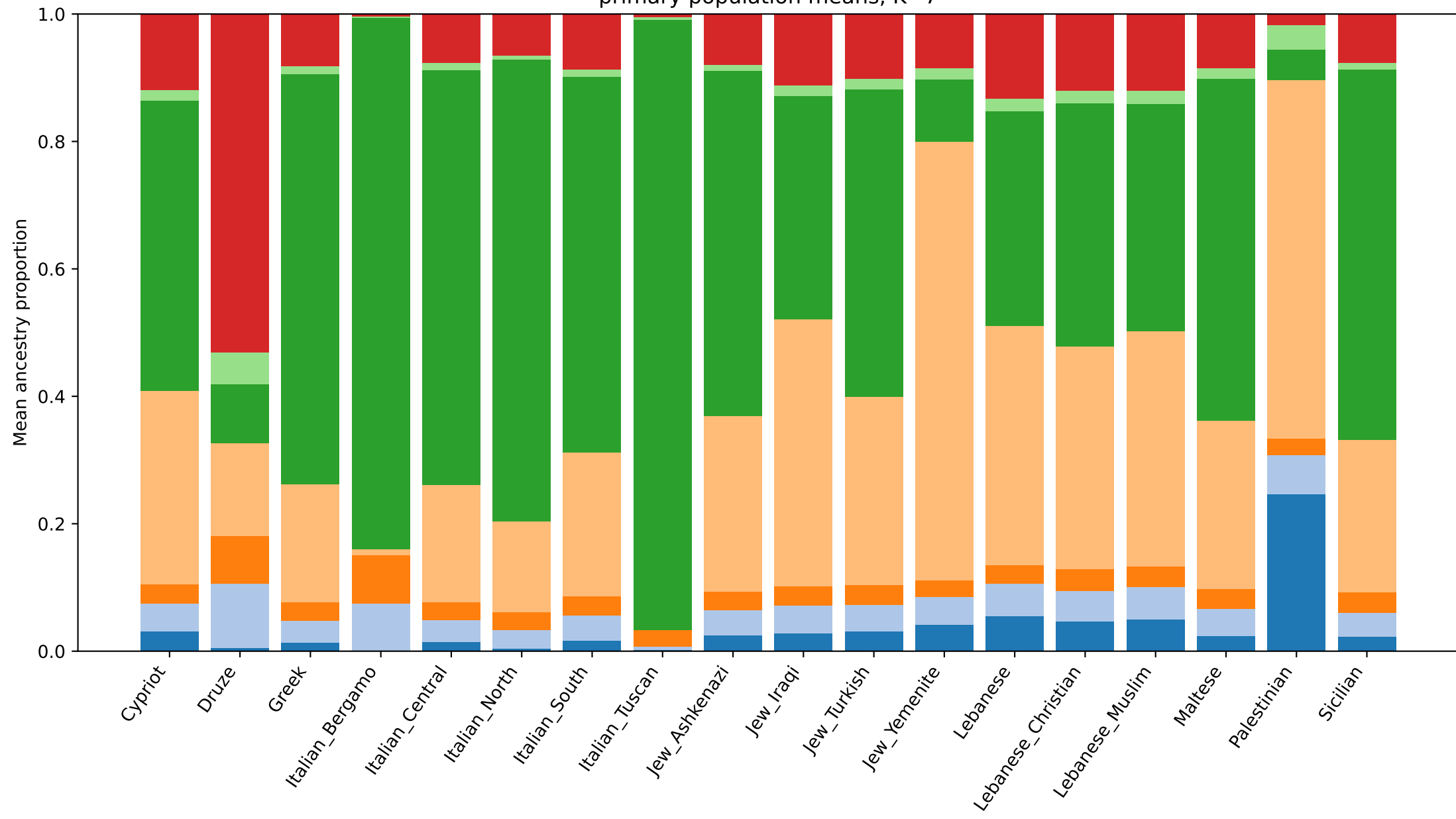
primary population means, K=7
