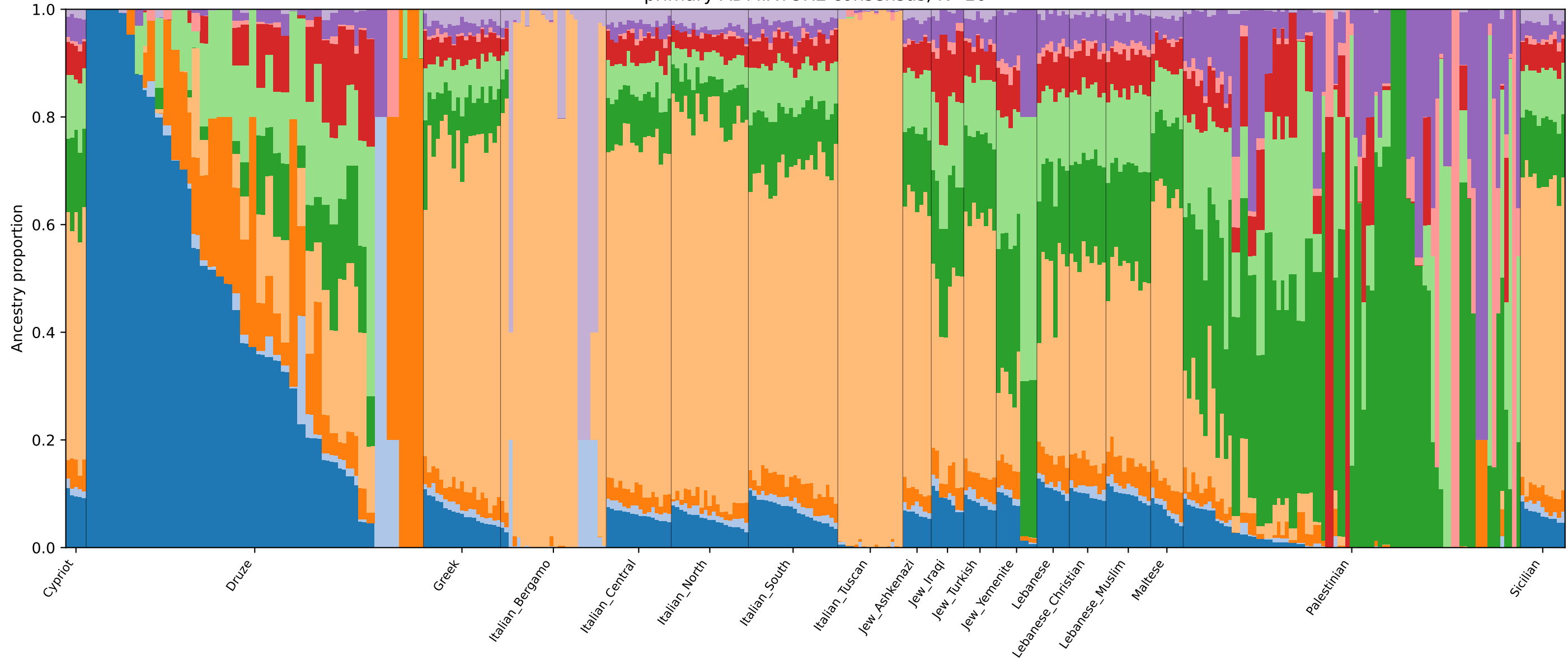
primary ADMIXTURE consensus, K=10
