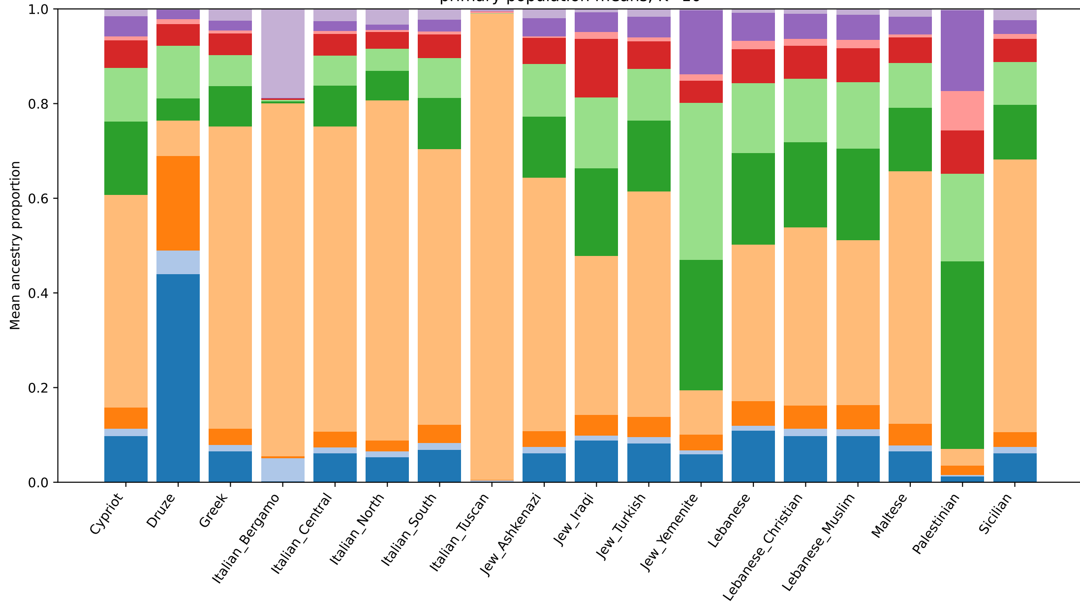
primary population means, K=10
