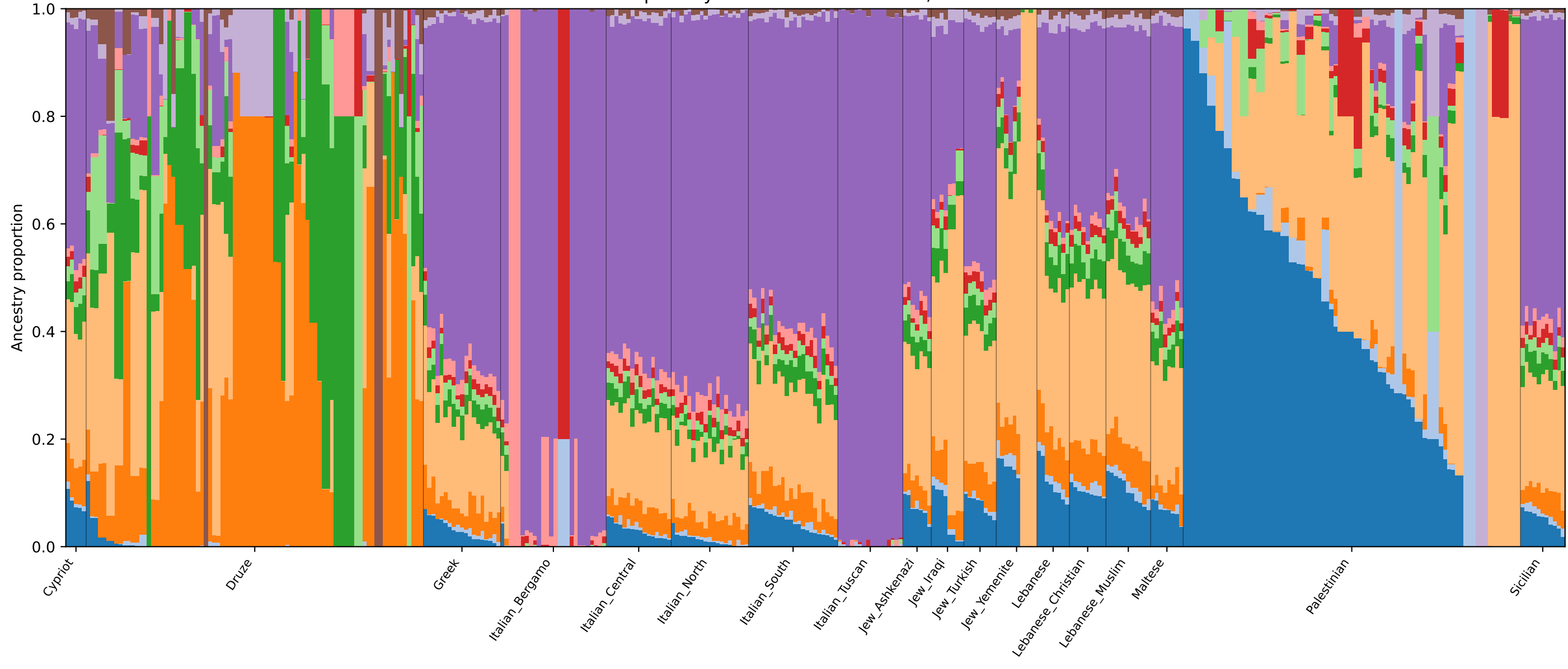
primary ADMIXTURE consensus, K=11
