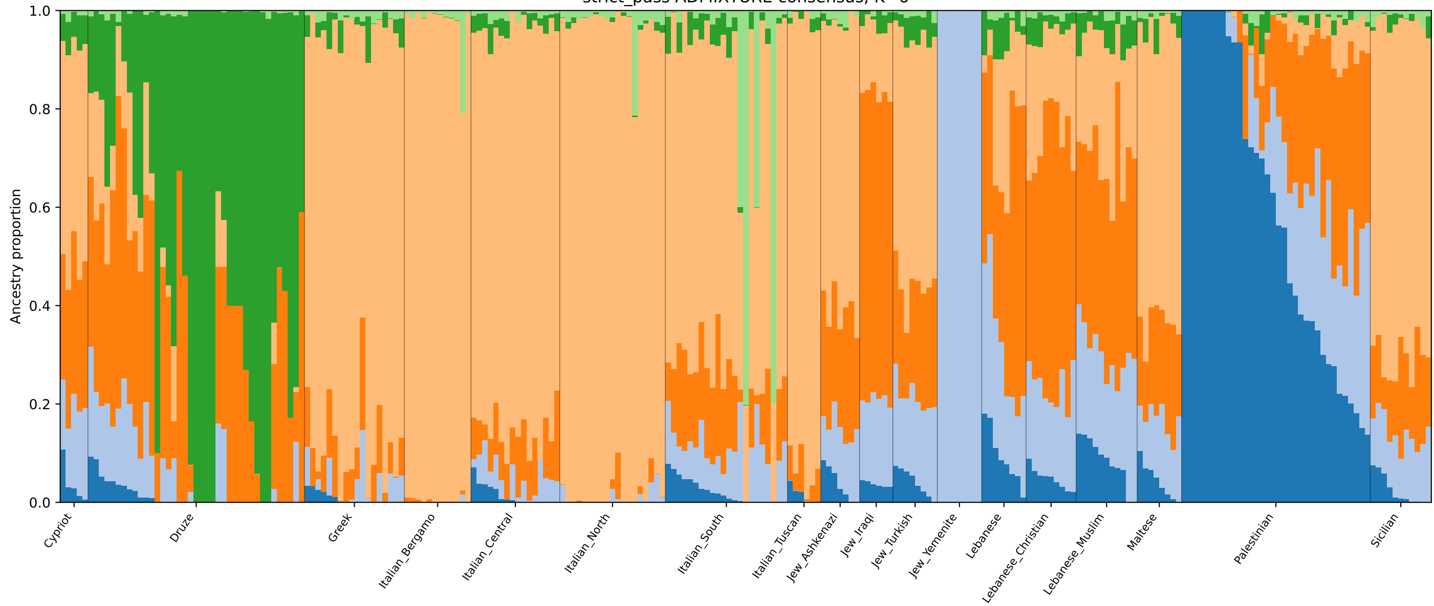
strict_pass ADMIXTURE consensus, K=6
