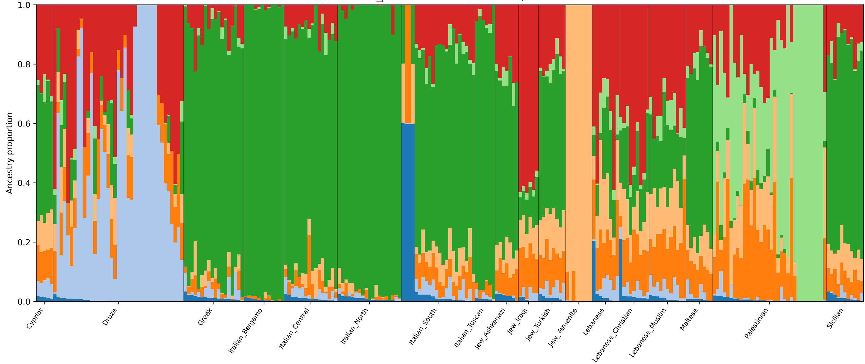
strict_pass ADMIXTURE consensus, K=7
