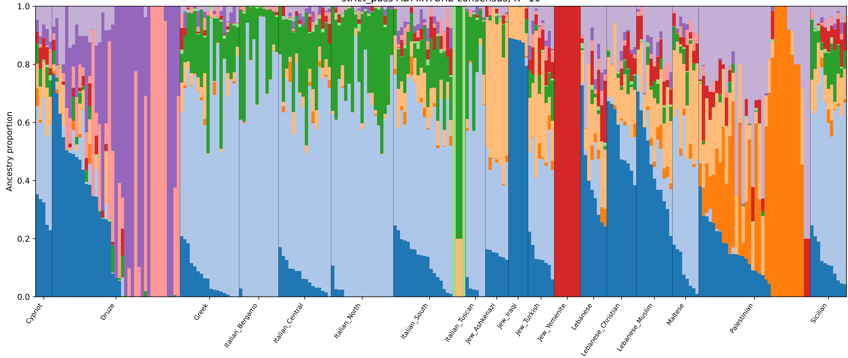
strict_pass ADMIXTURE consensus, K=10
