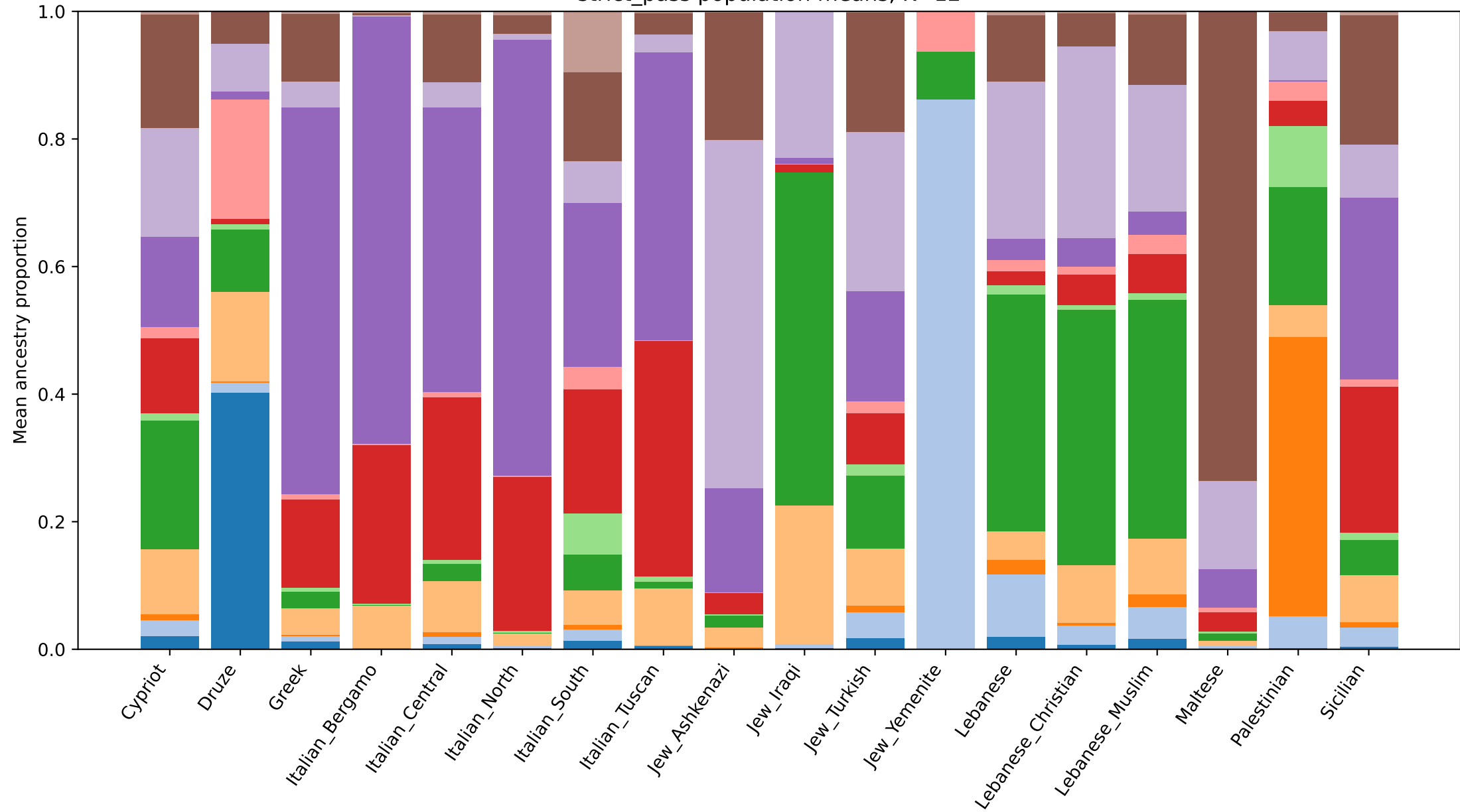
strict_pass population means, K=12
