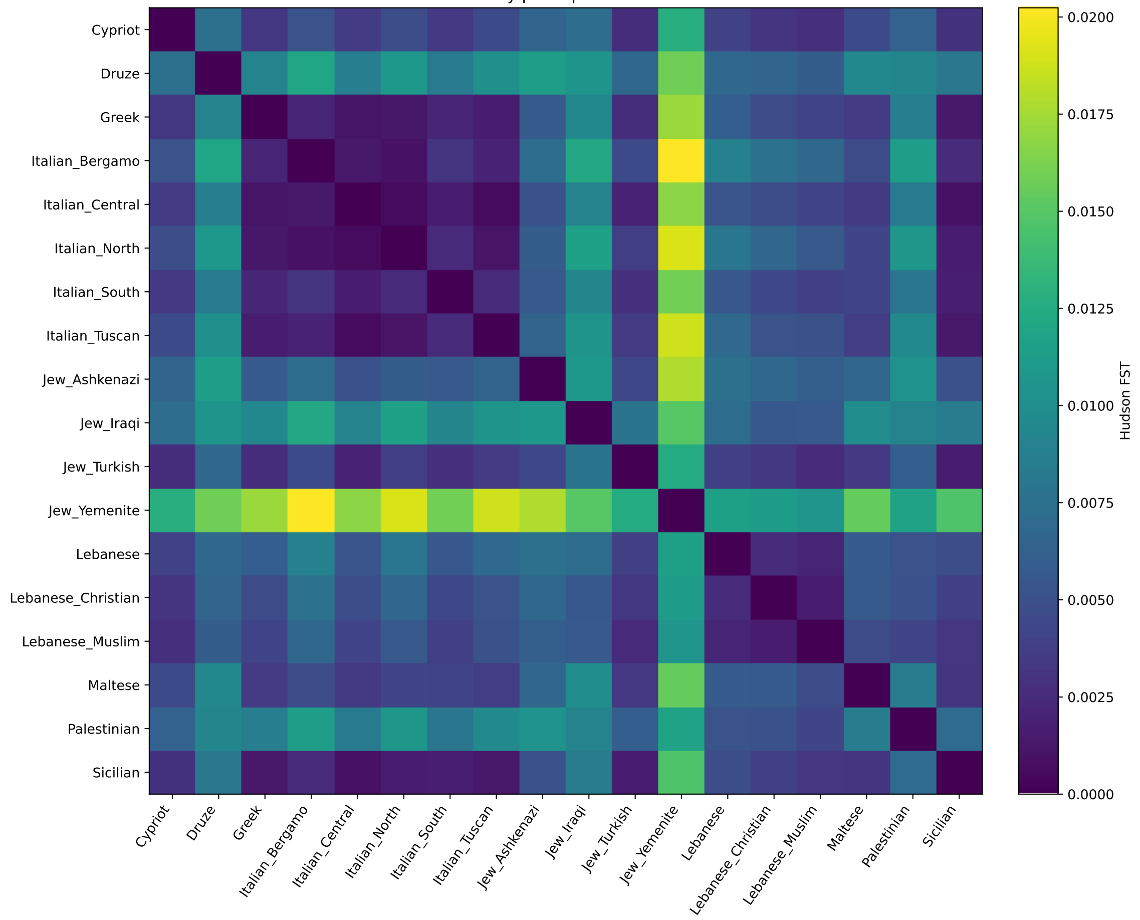
Strict Pass-only panel pairwise Hudson FST
