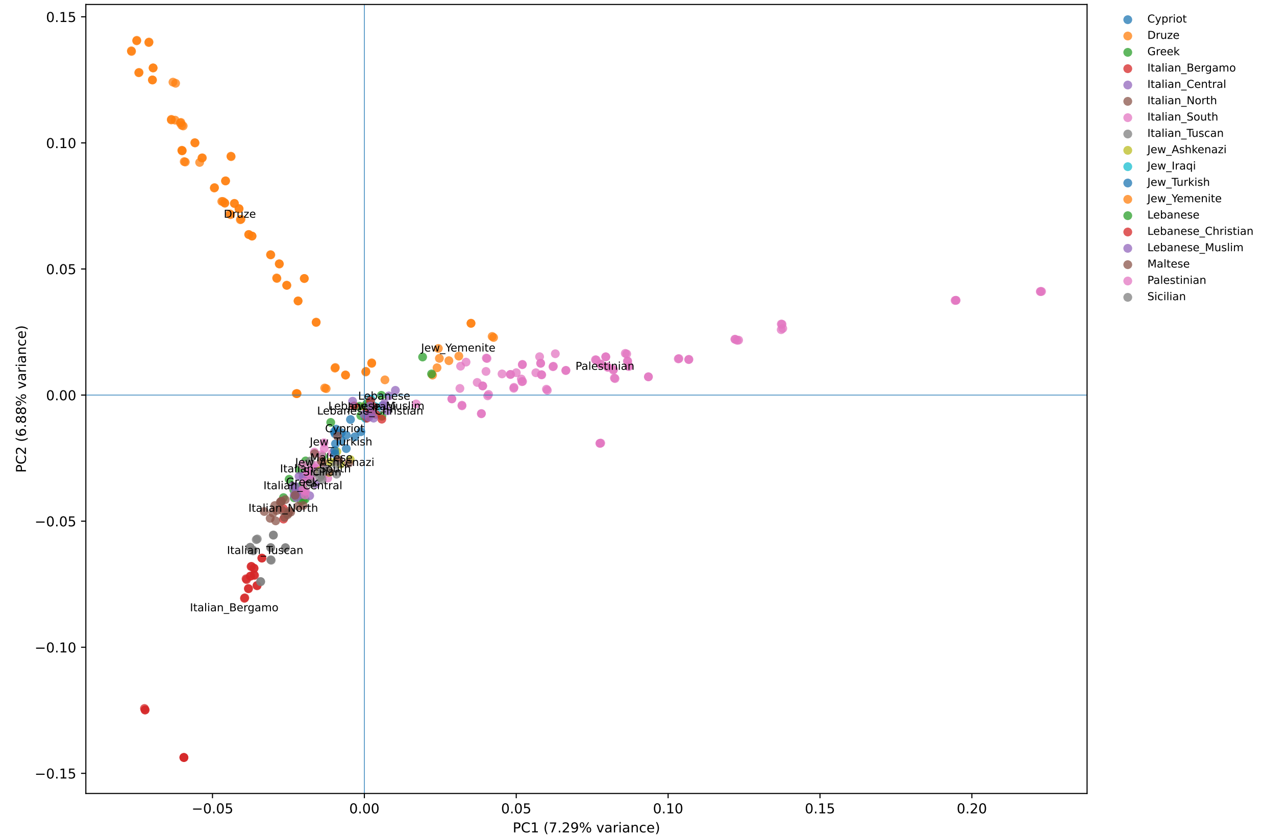
Primary PCA: PC1 vs PC2
