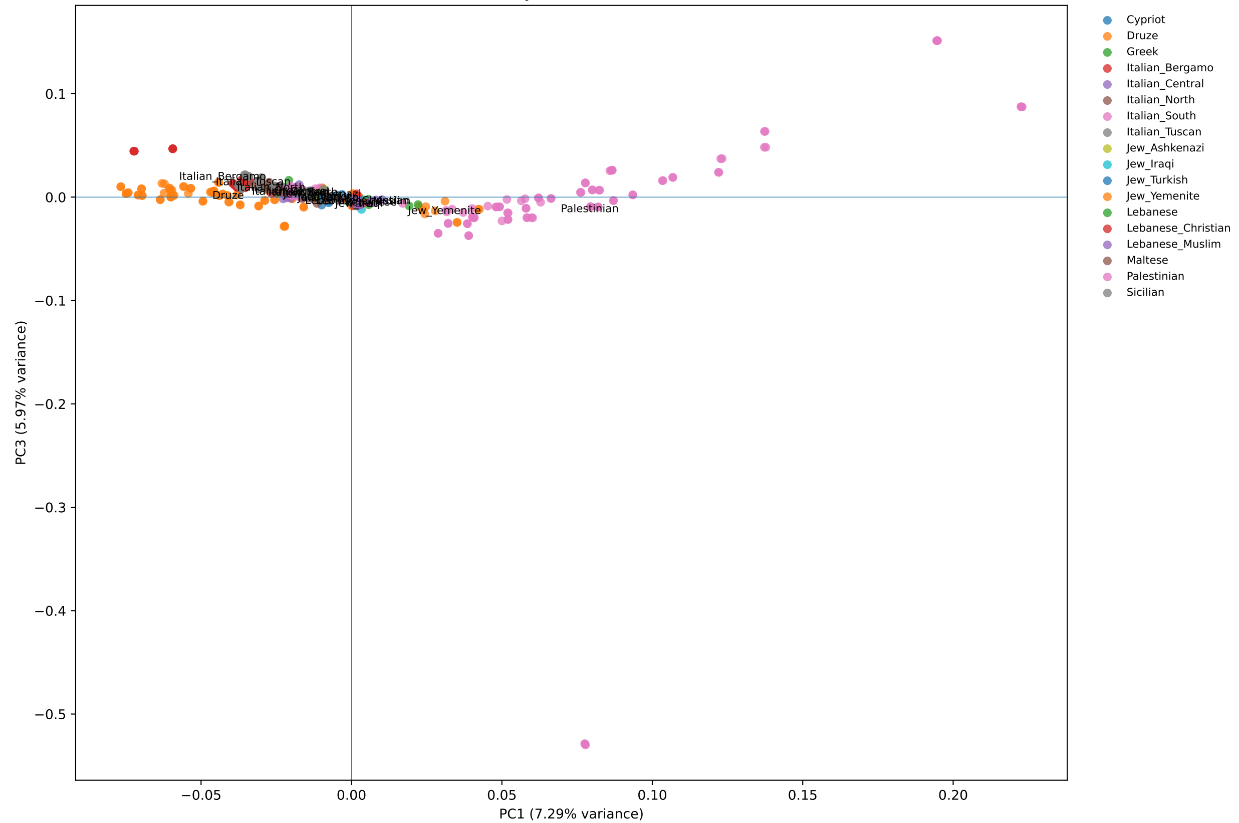
Primary PCA: PC1 vs PC3
