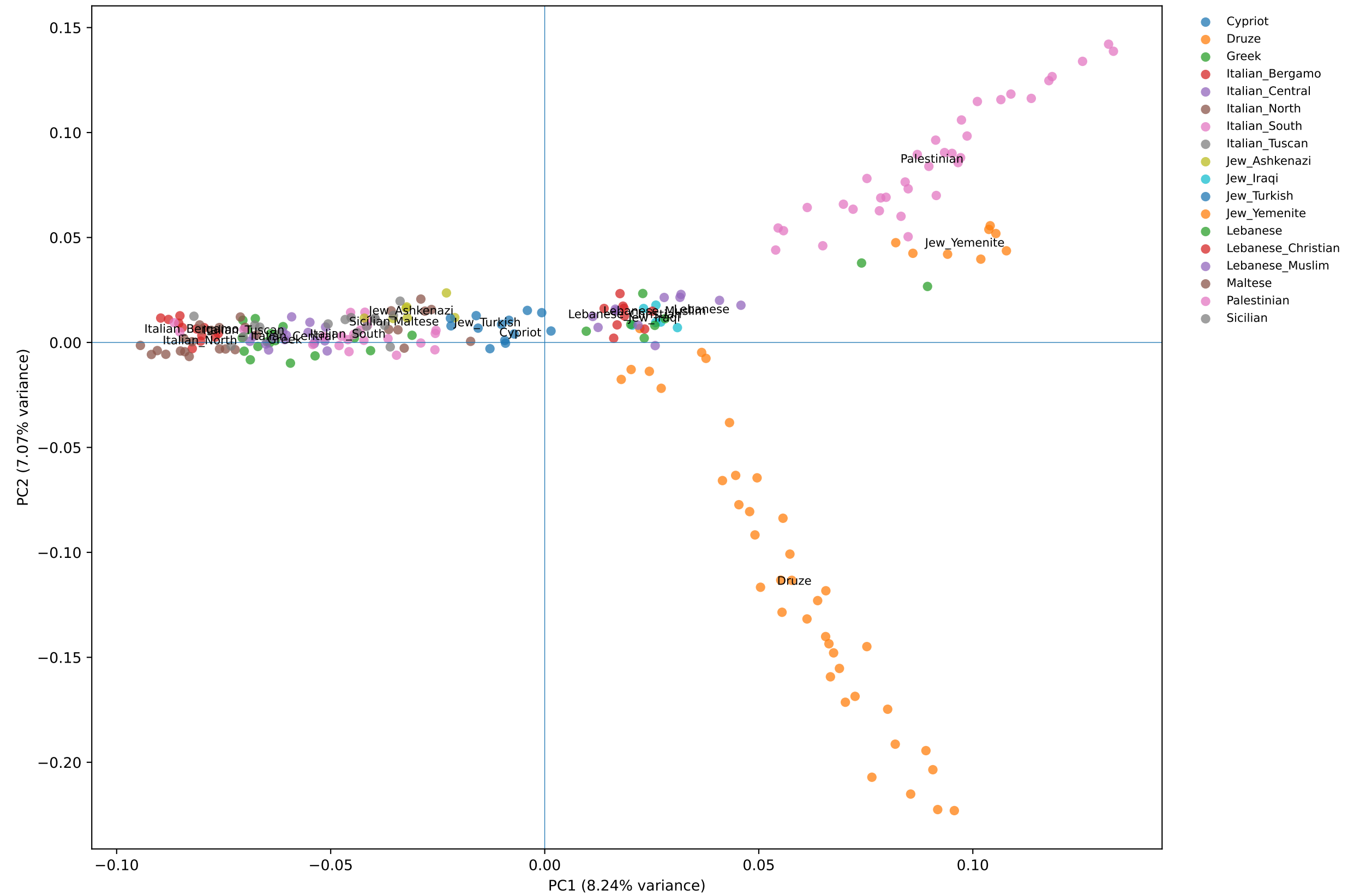
Strict Pass PCA: PC1 vs PC2
