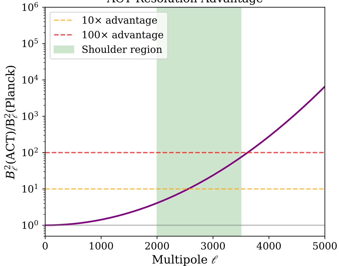
ACT Resolution Advantage
