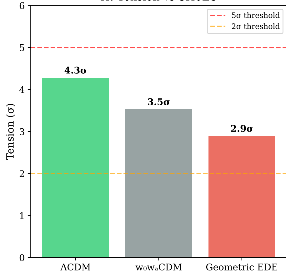
H 0 Tension vs SH0ES
