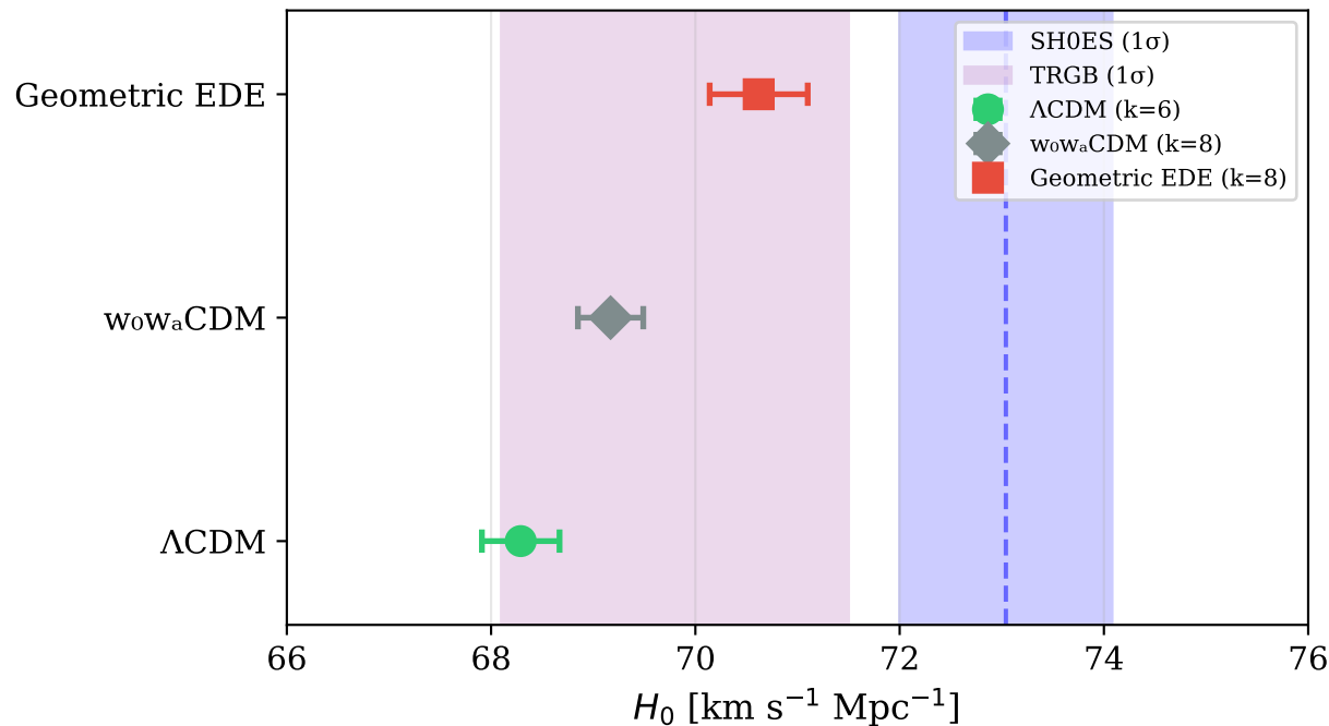
Hubble Constant Constraints
