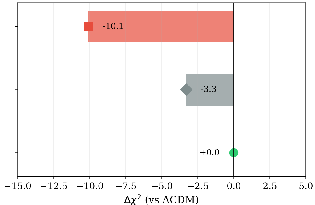
Goodness of Fit
