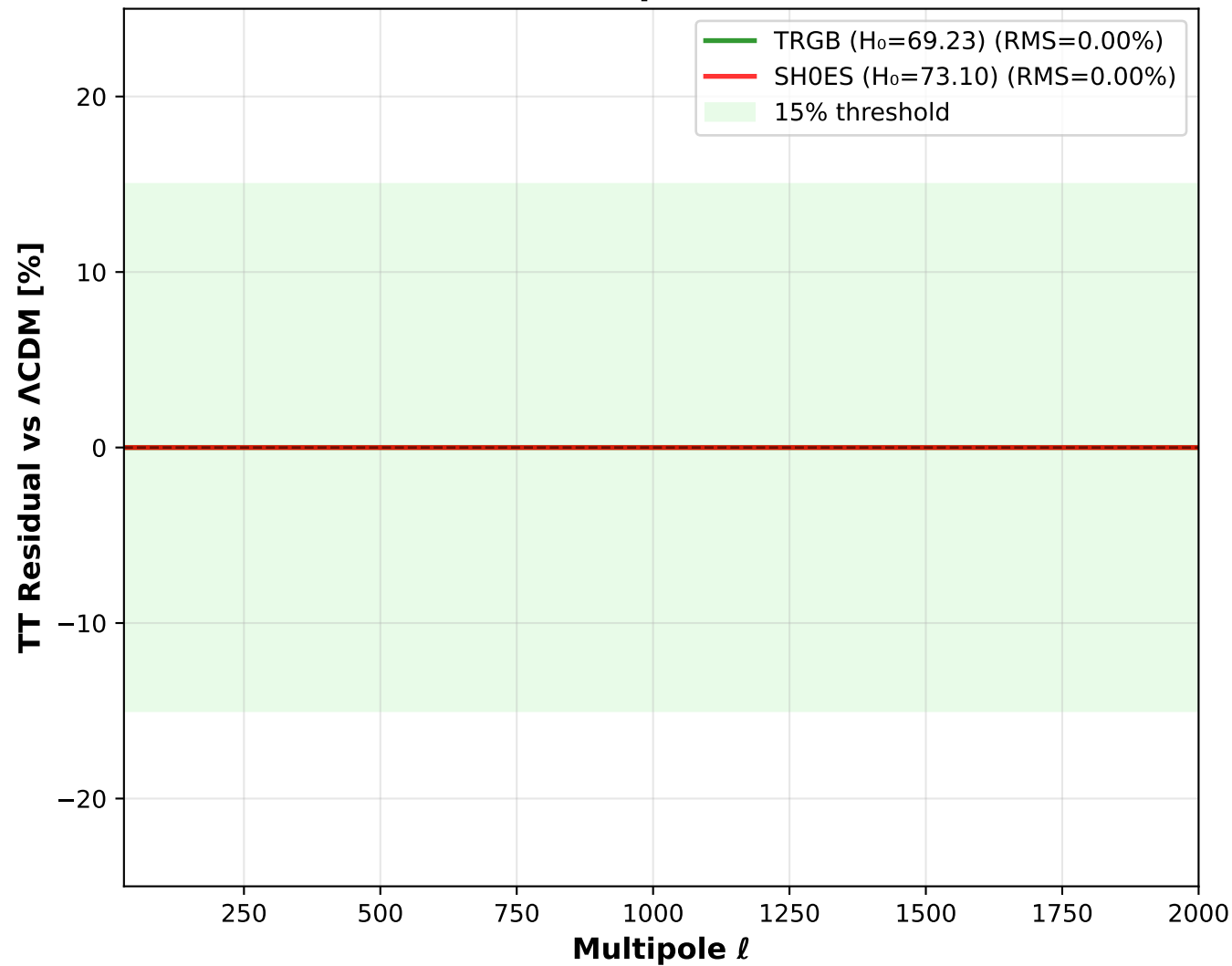
CMB TT Power Spectrum Residuals
