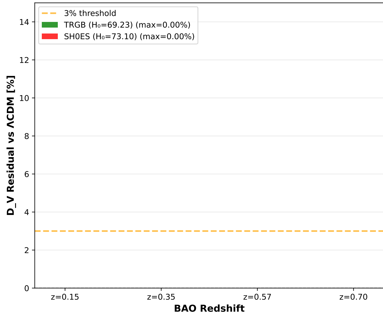
BAO Distance Residuals
