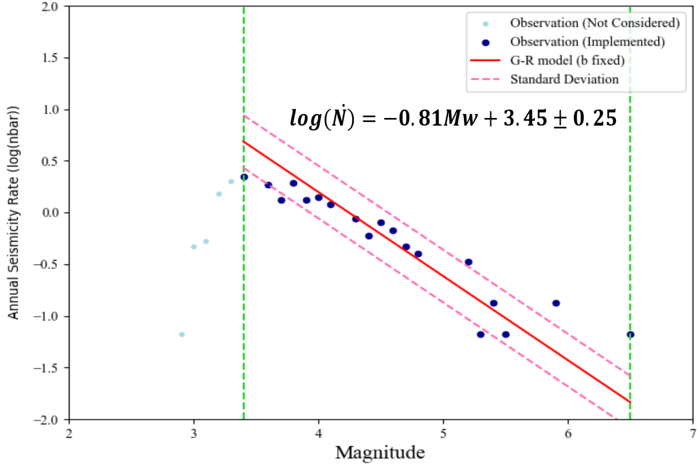
Magnitude–frequency distribution used for a-value estimation in Zone 1 (Grünthal pers. comm.)
