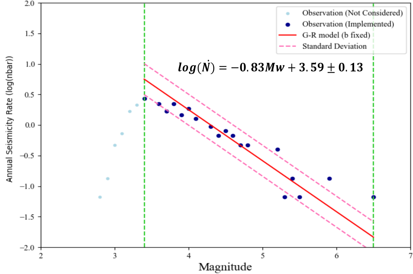
Magnitude–frequency distribution used for a-value estimation in Zone 1 (Gardner & Knopoff, 1974)
