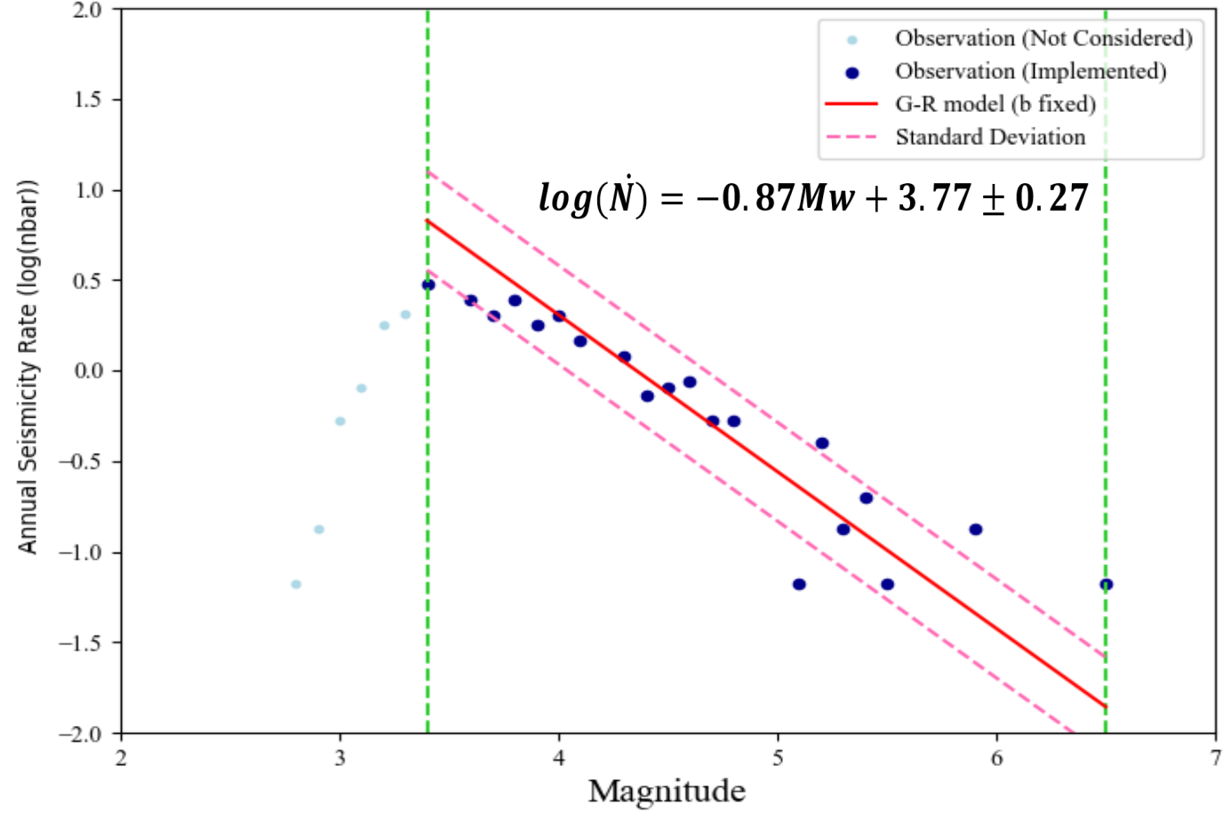
Magnitude–frequency distribution used for a-value estimation in Zone 1 (Uhrhammer, 1986)
