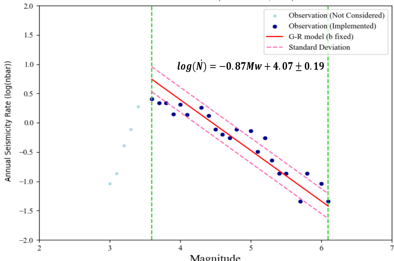
Magnitude–frequency distribution used for a-value estimation in Zone 2 (Uhrhammer, 1986)
