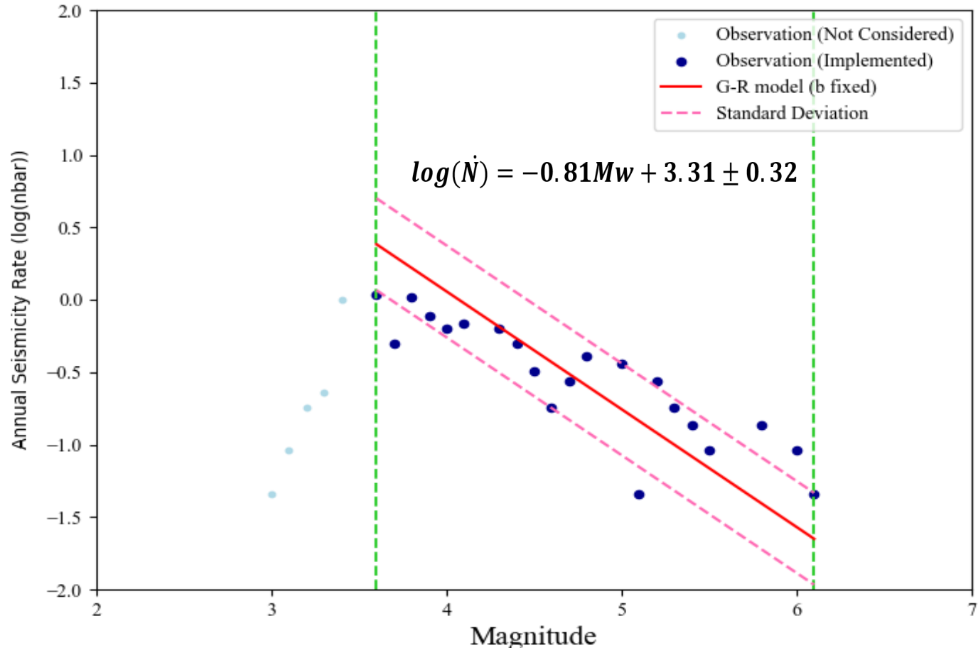
Magnitude–frequency distribution used for a-value estimation in Zone 2 (Grünthal pers. comm.)
