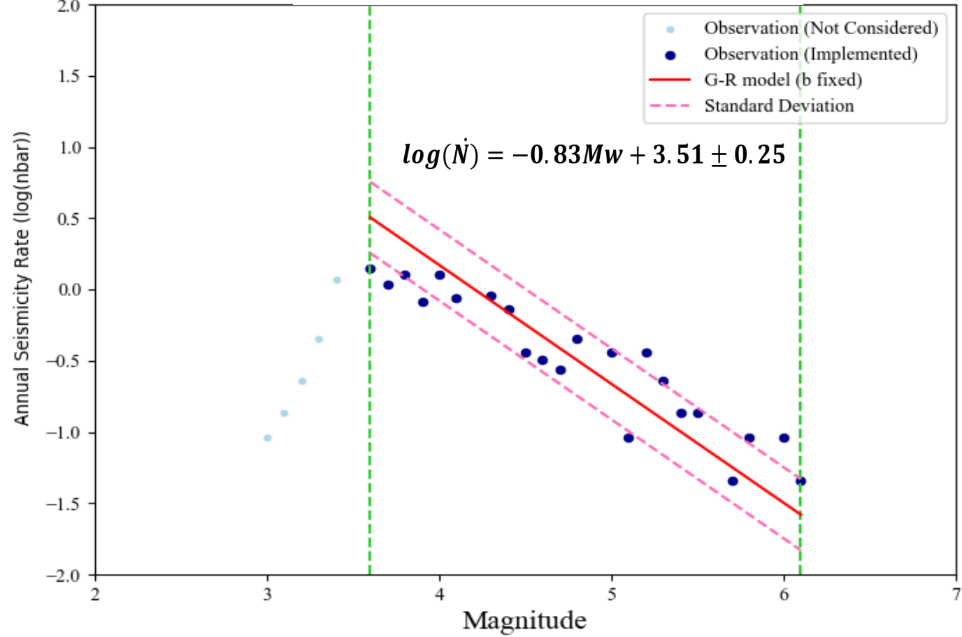
Magnitude–frequency distribution used for a-value estimation in Zone 2 (Gardner & Knopoff, 1974)
