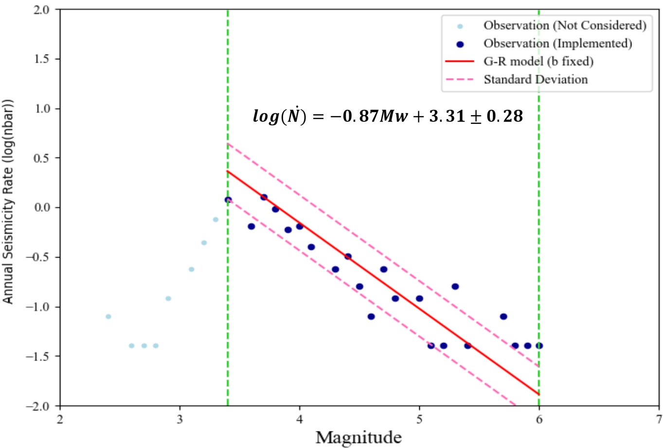
Magnitude–frequency distribution used for a-value estimation in Zone 3 (Uhrhammer, 1986)
