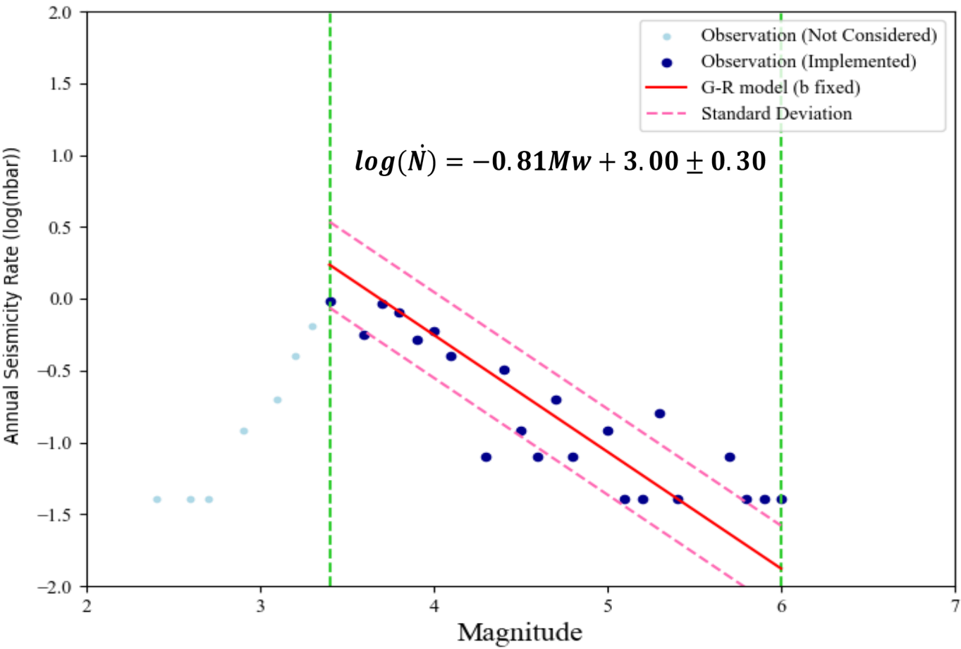
Magnitude–frequency distribution used for a-value estimation in Zone 3 (Grünthal pers. comm.)
