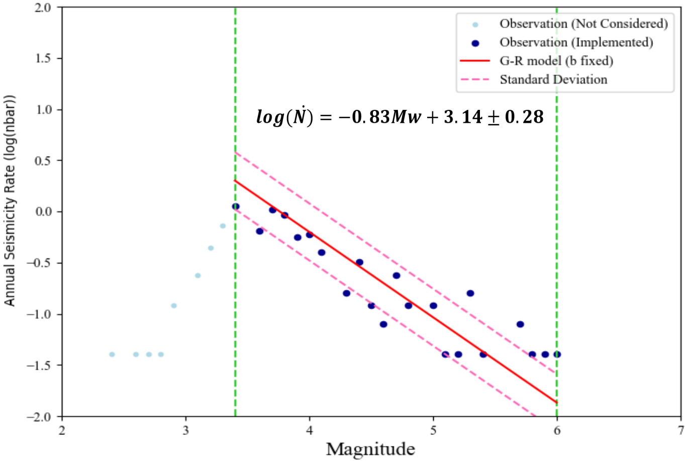
Magnitude–frequency distribution used for a-value estimation in Zone 3 (Gardner & Knopoff, 1974)
