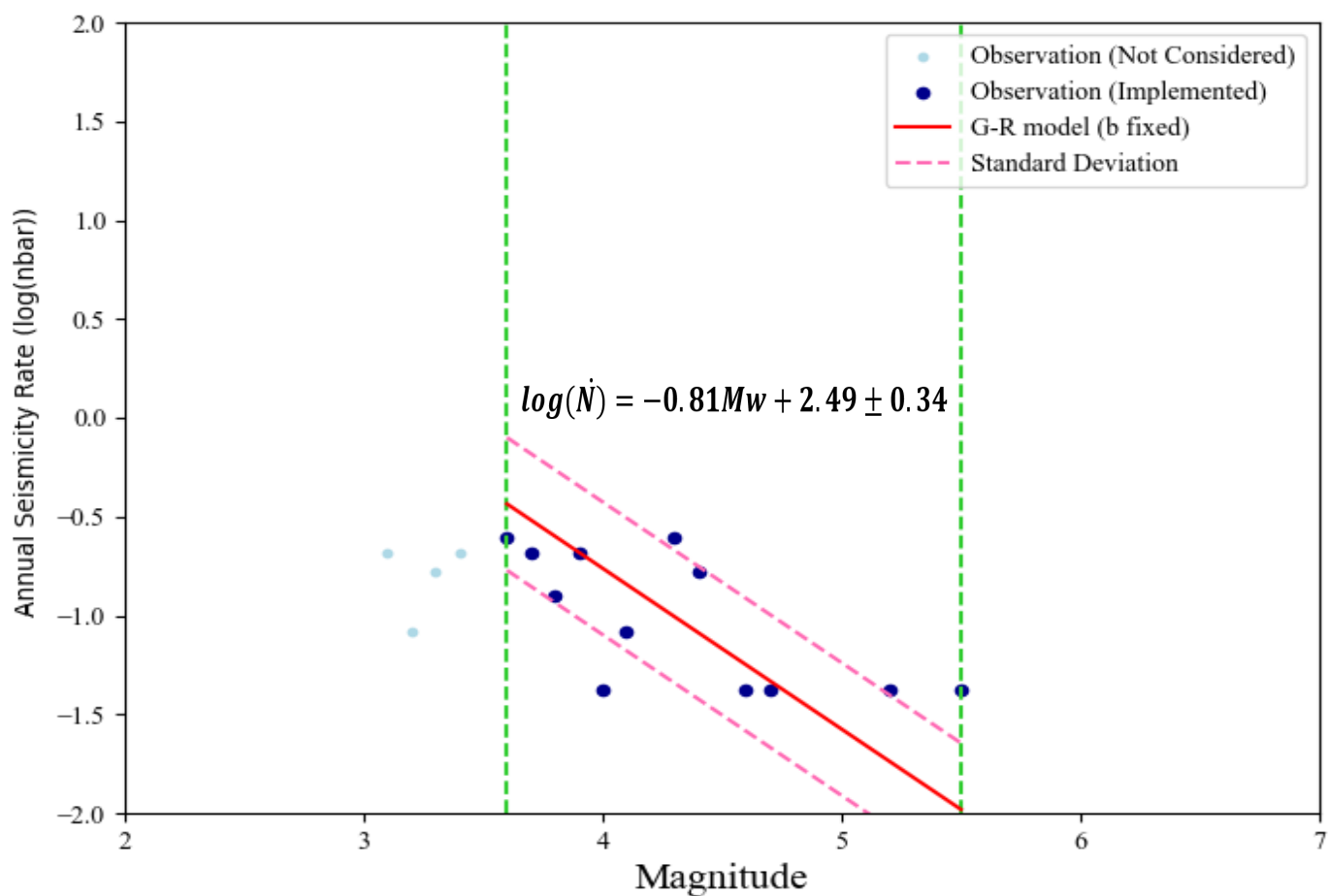
Magnitude–frequency distribution used for a-value estimation in Zone 4 (Grünthal pers. comm.)
