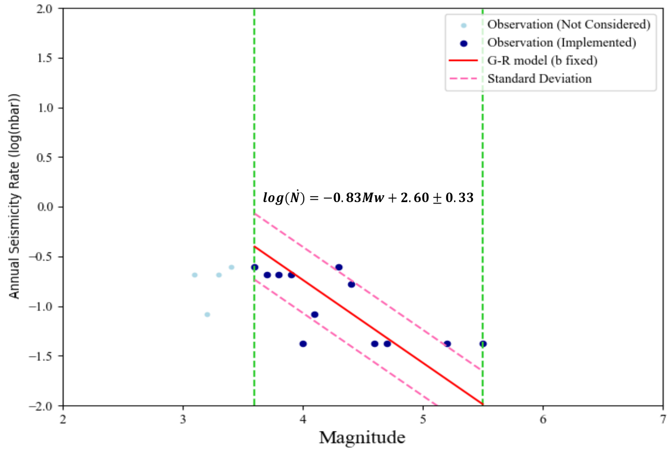
Magnitude–frequency distribution used for a-value estimation in Zone 4 (Gardner & Knopoff, 1974)
