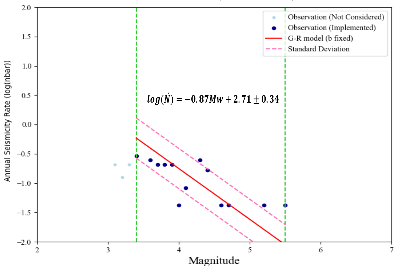
Magnitude–frequency distribution used for a-value estimation in Zone 4 (Uhrhammer, 1986)
