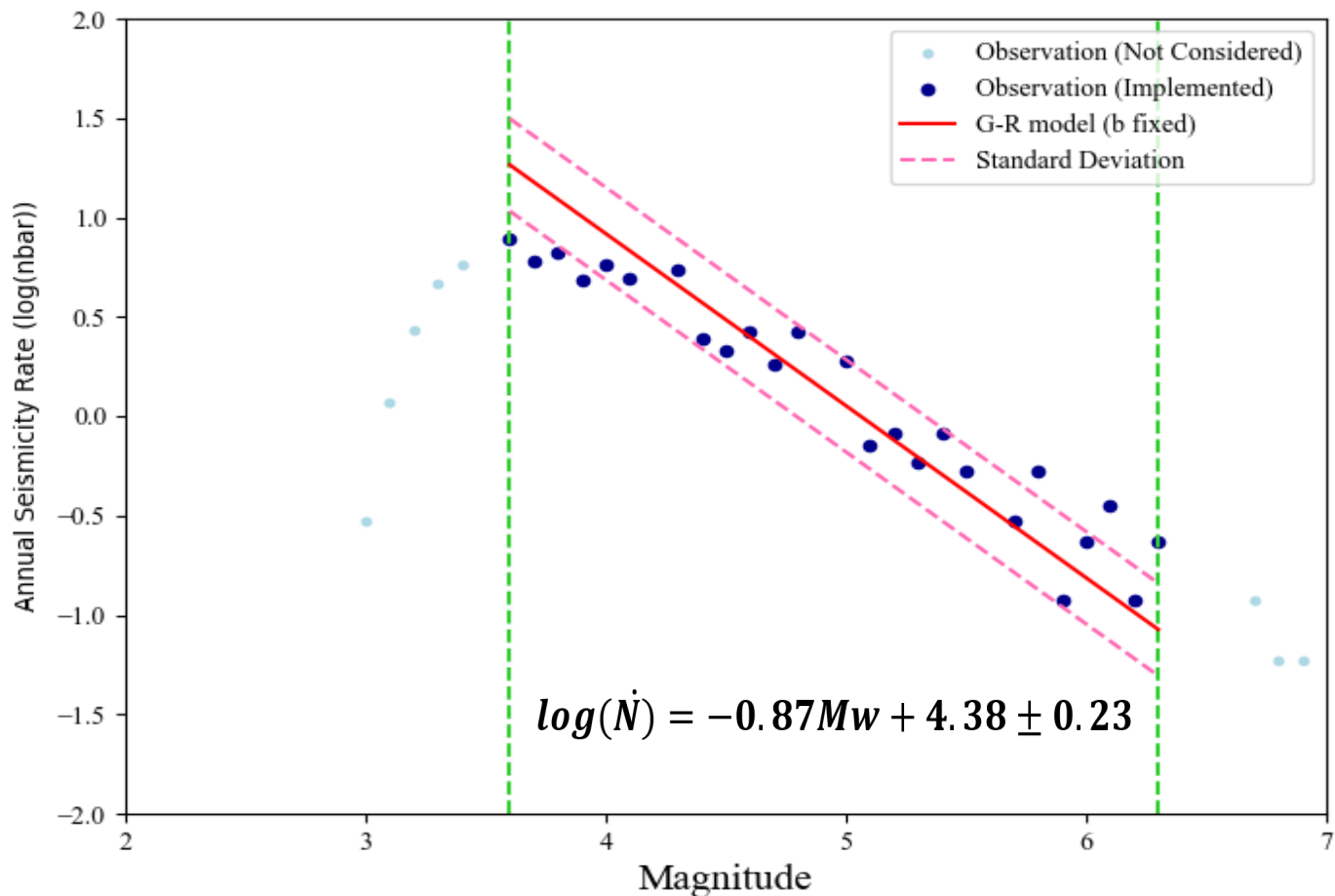
Magnitude–frequency distribution used for a-value estimation in Zone 5 (Uhrhammer, 1986)
