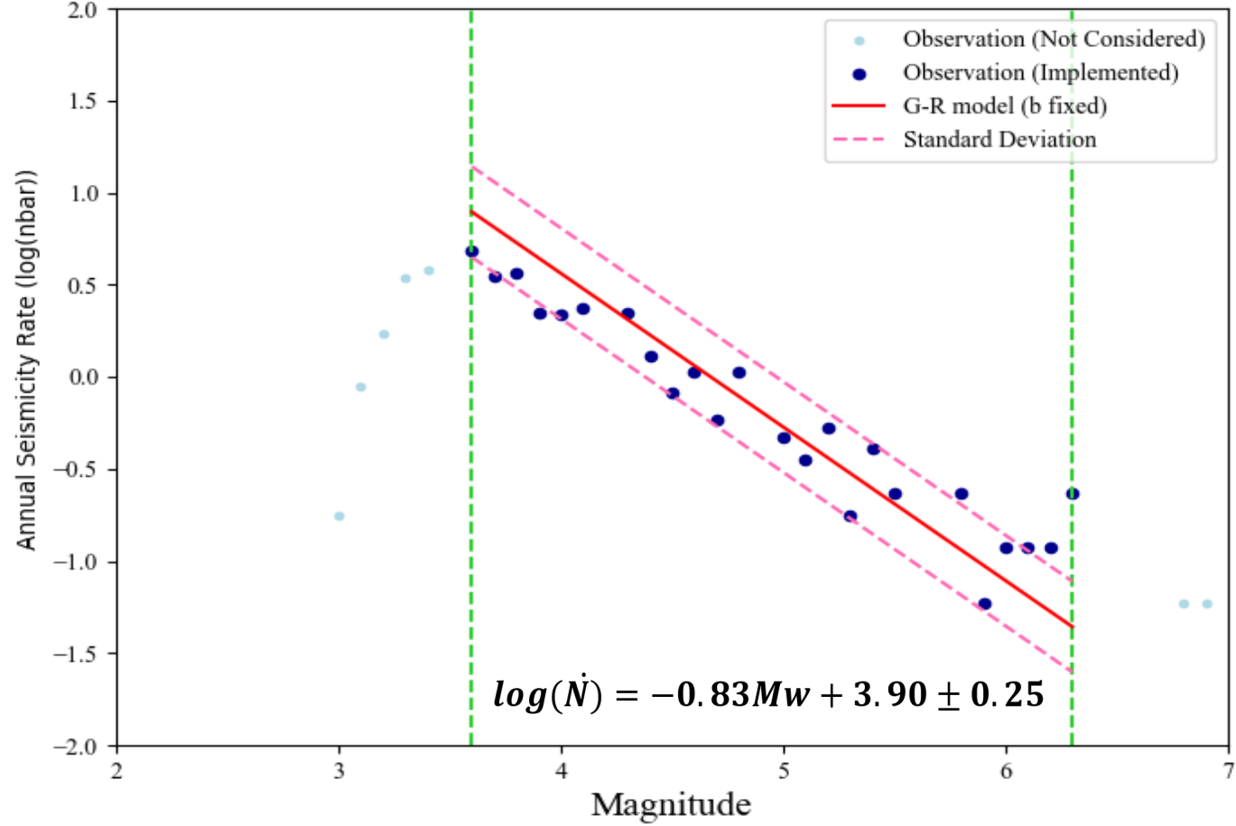
Magnitude–frequency distribution used for a-value estimation in Zone 5 (Gardner & Knopoff, 1974)
