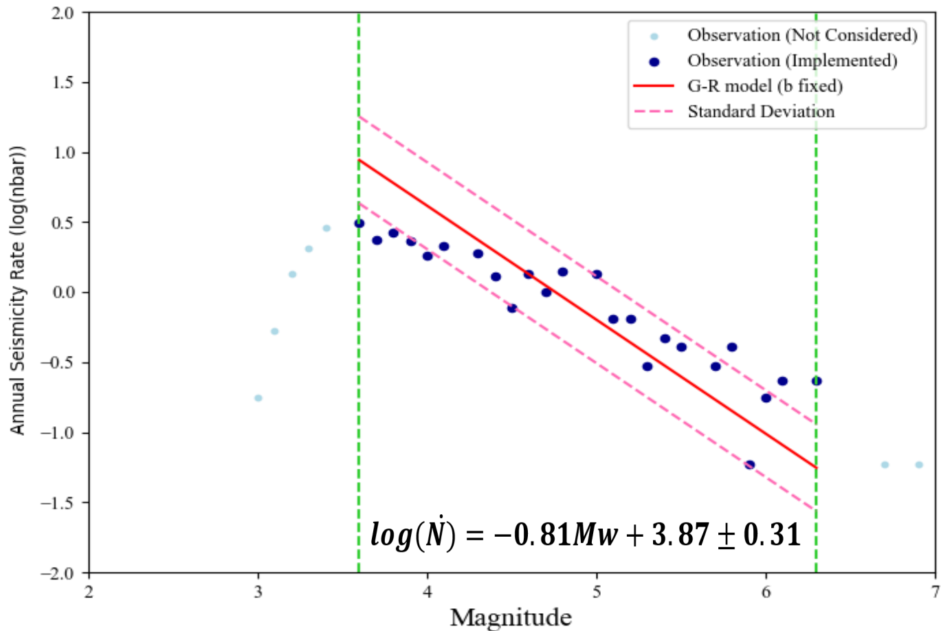
Magnitude–frequency distribution used for a-value estimation in Zone 5 (Grünthal pers. comm.)
