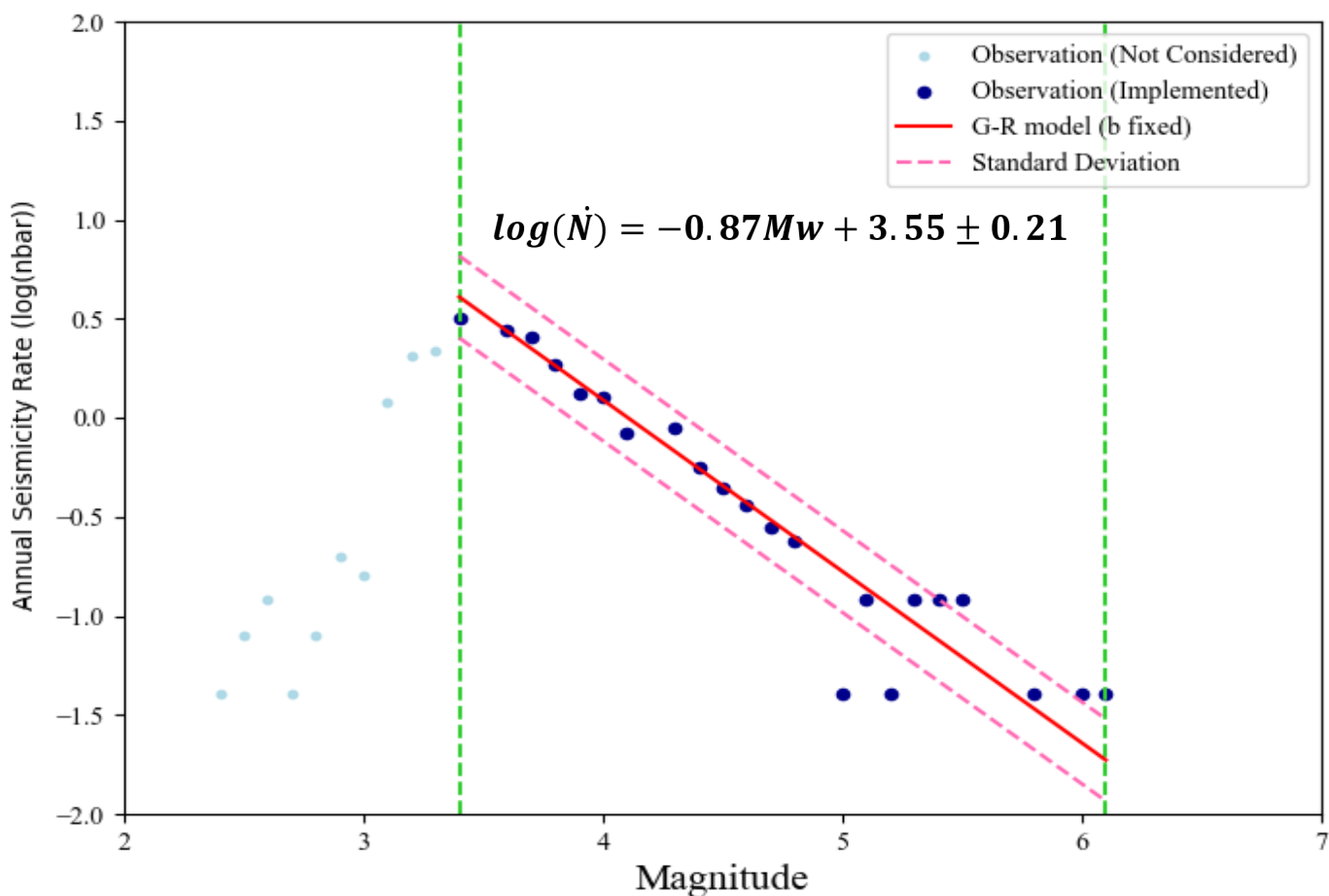
Magnitude–frequency distribution used for a-value estimation in Zone 6 (Uhrhammer, 1986)
