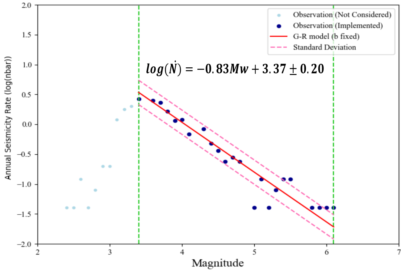
Magnitude–frequency distribution used for a-value estimation in Zone 6 (Gardner & Knopoff, 1974)
