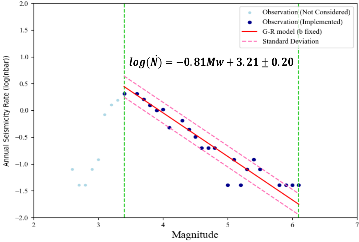
Magnitude–frequency distribution used for a-value estimation in Zone 6 (Grünthal pers. comm.)
