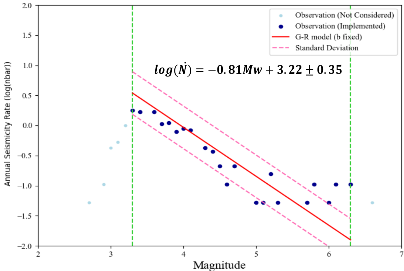
Magnitude–frequency distribution used for a-value estimation in Zone 7 (Grünthal pers. comm.)
