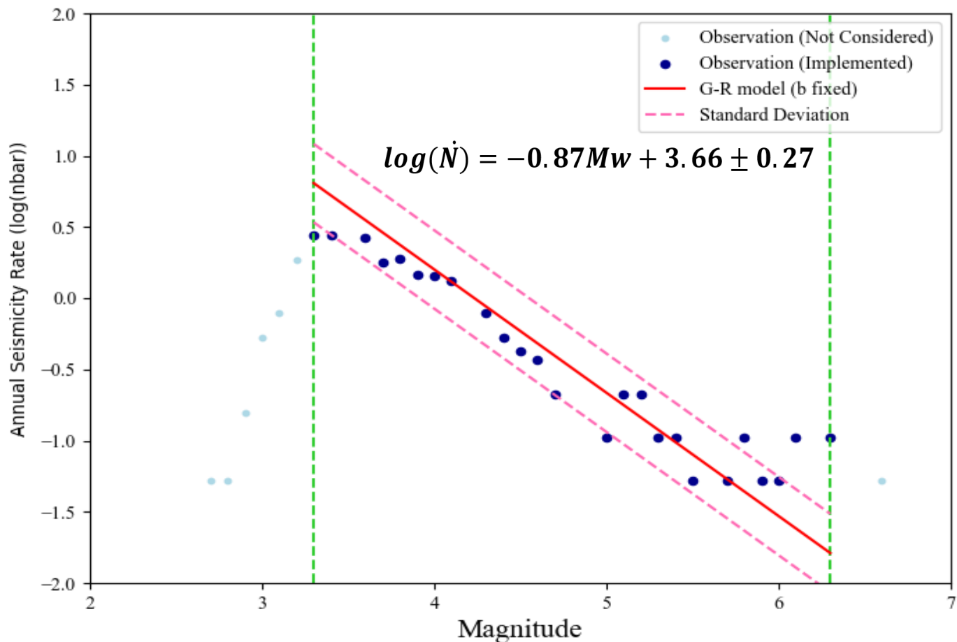
Magnitude–frequency distribution used for a-value estimation in Zone 7 (Uhrhammer, 1986)
