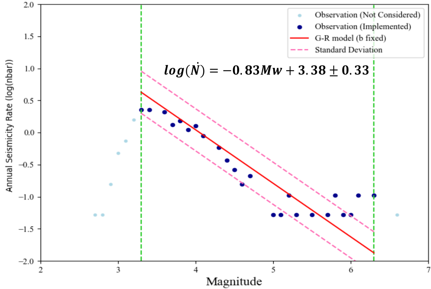
Magnitude–frequency distribution used for a-value estimation in Zone 7 (Gardner & Knopoff, 1974)
