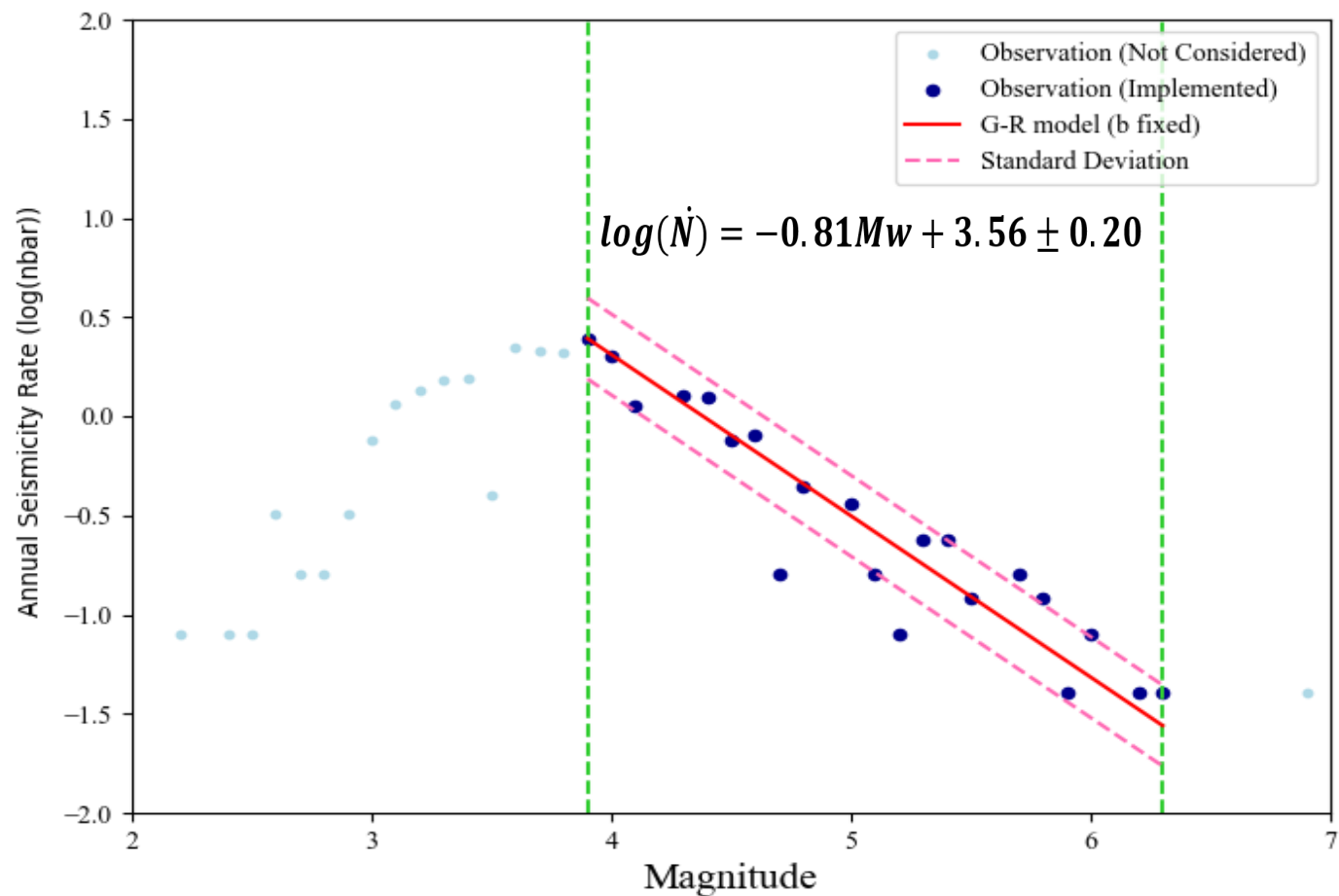
Magnitude–frequency distribution used for a-value estimation in Zone 8 (Grünthal pers. comm.)
