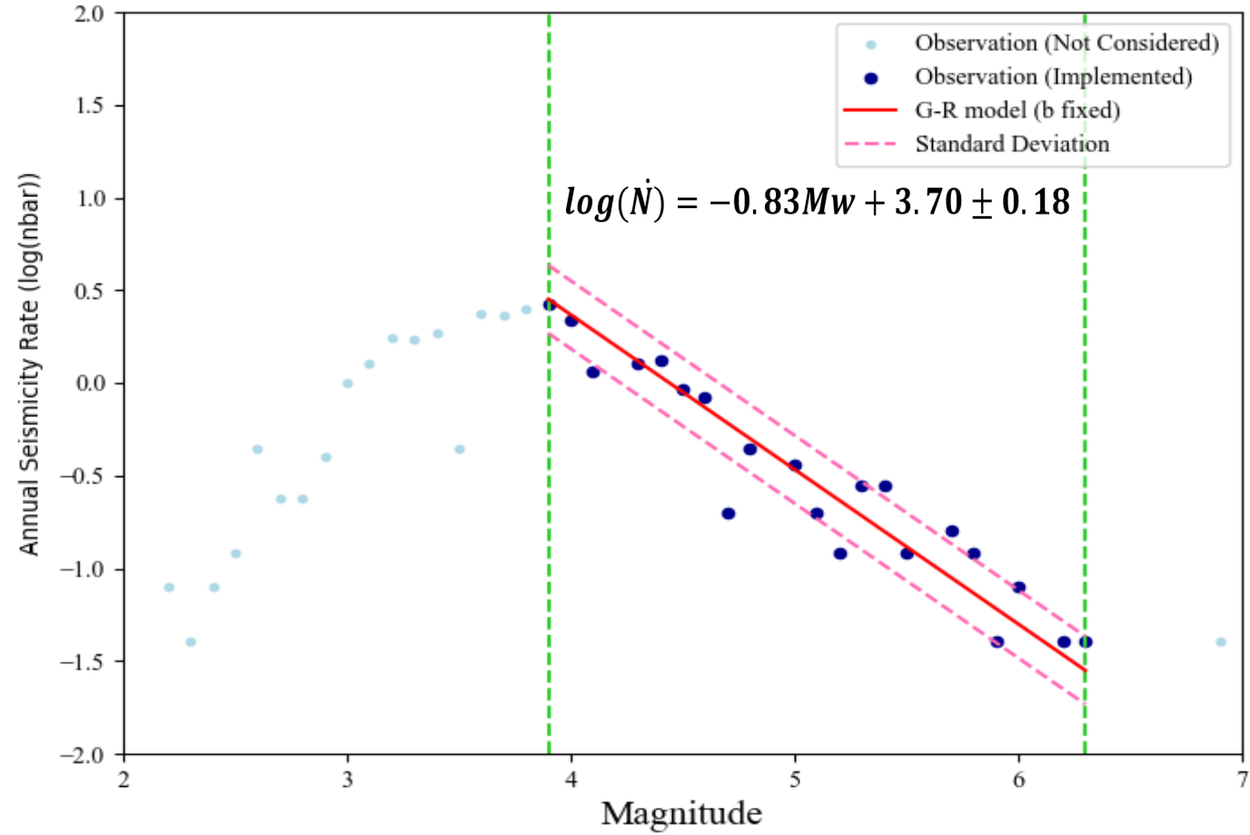
Magnitude–frequency distribution used for a-value estimation in Zone 8 (Gardner & Knopoff, 1974)
