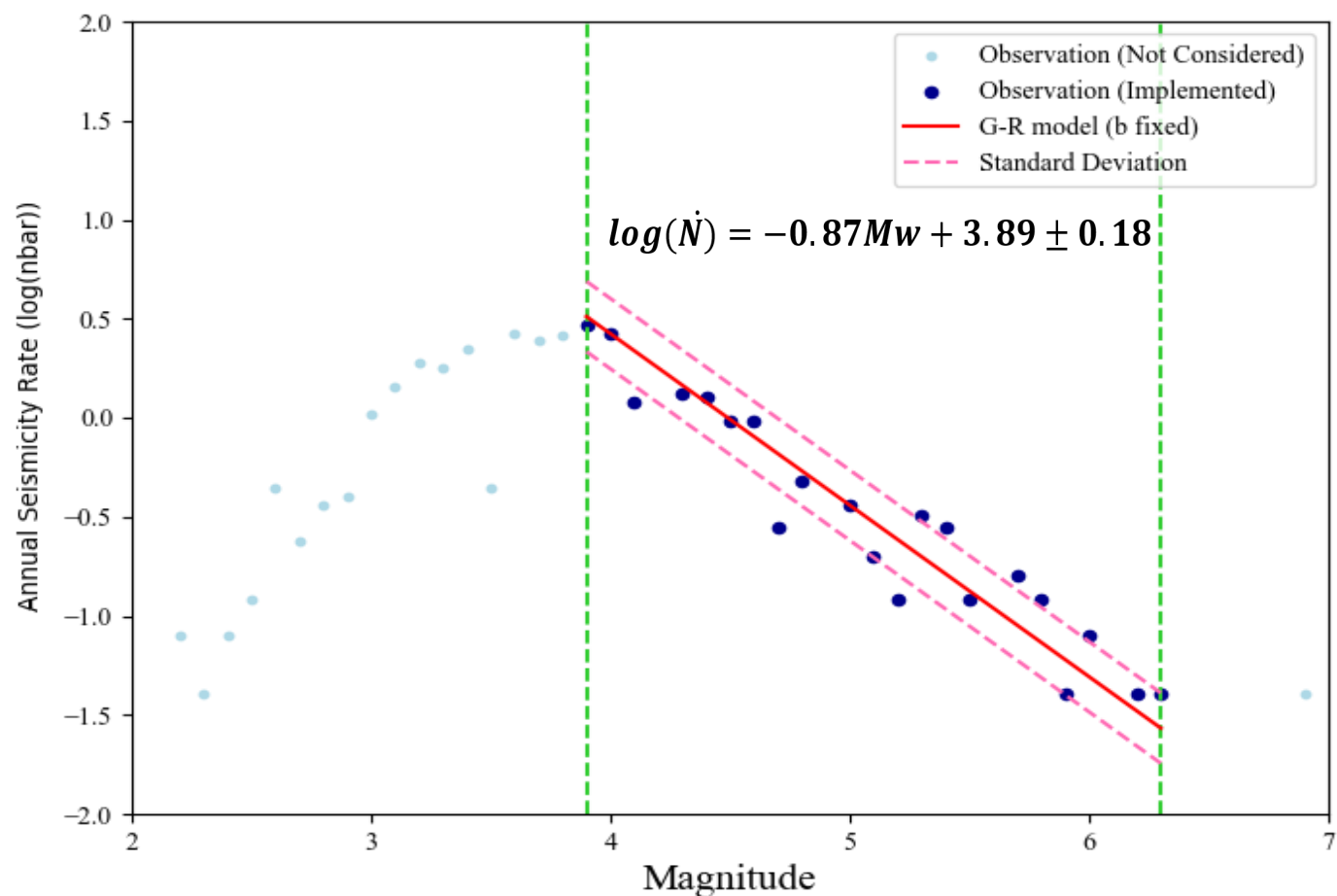
Magnitude–frequency distribution used for a-value estimation in Zone 8 (Uhrhammer, 1986)
