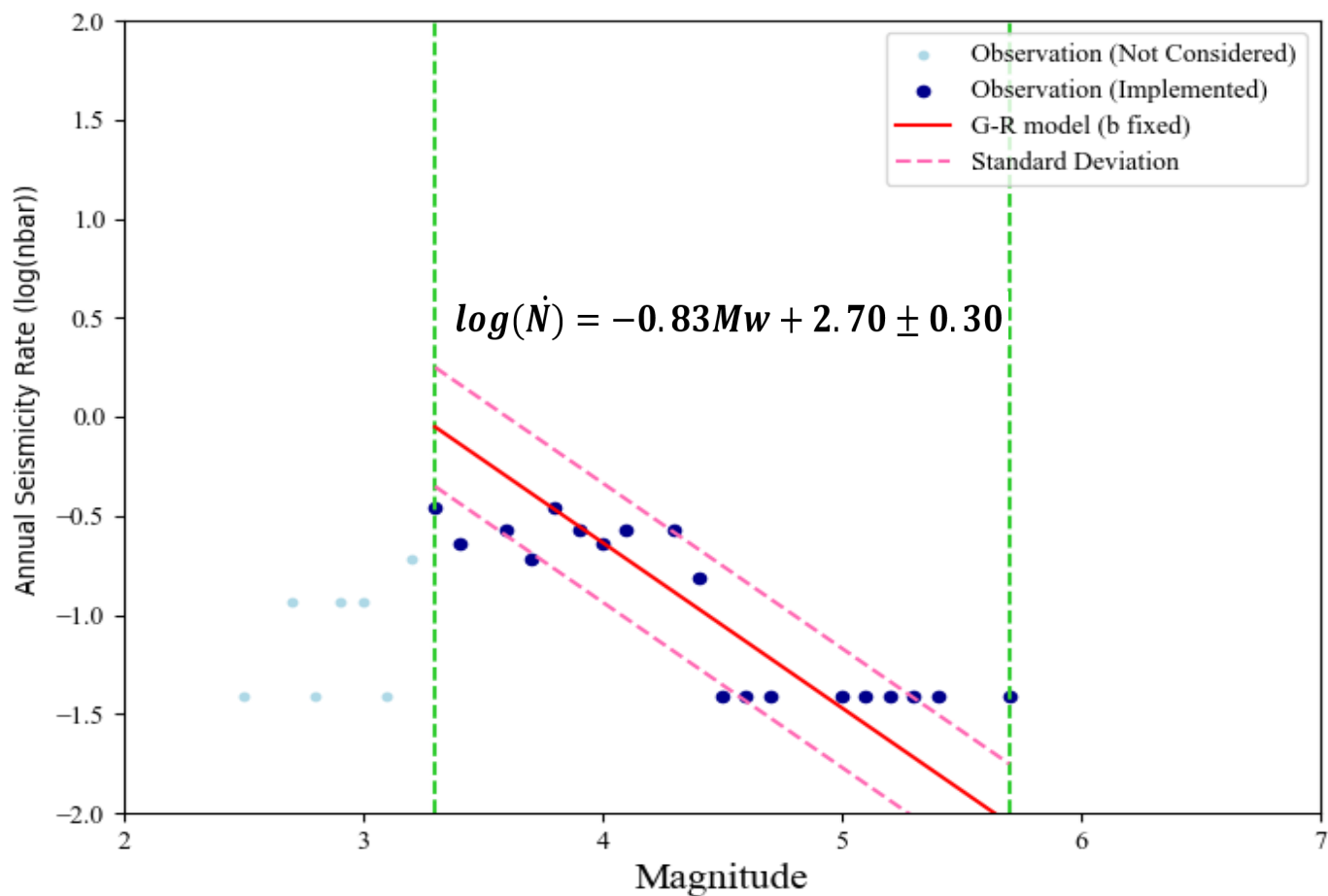
Magnitude–frequency distribution used for a-value estimation in Zone 9 (Gardner & Knopoff, 1974)
