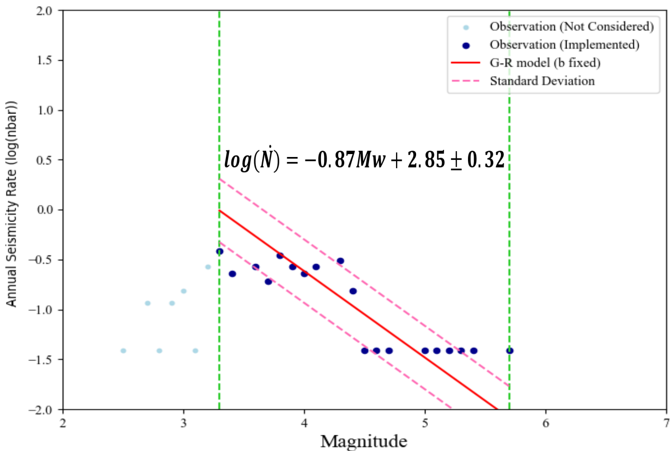
Magnitude–frequency distribution used for a-value estimation in Zone 9 (Uhrhammer, 1986)
