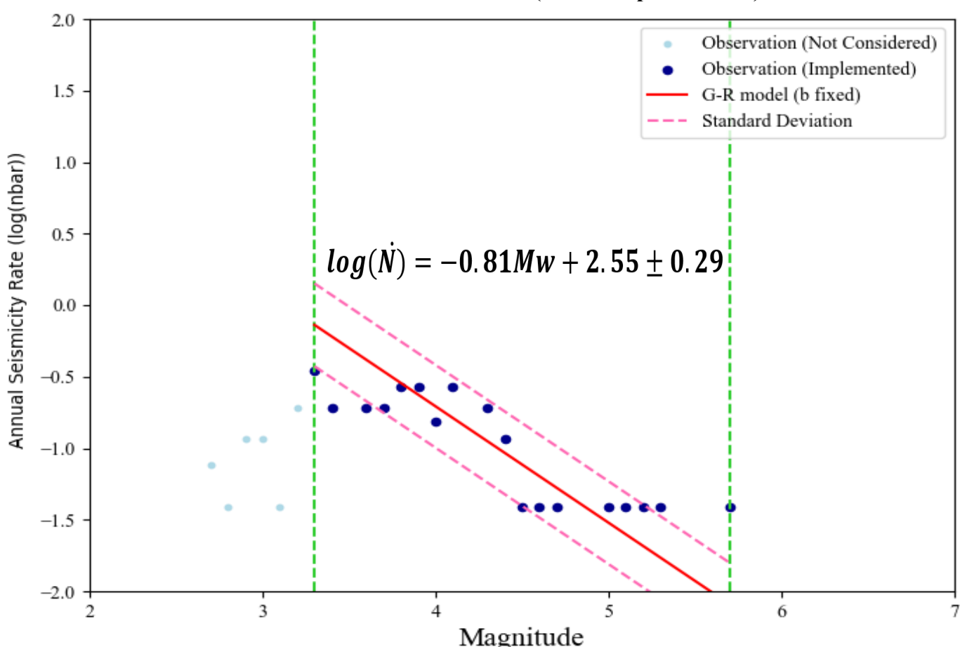
Magnitude–frequency distribution used for a-value estimation in Zone 9 (Grünthal pers. comm.)
